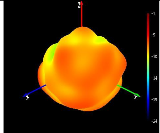
001# LTE antenna sample 3D orientation map (1960MHz)
