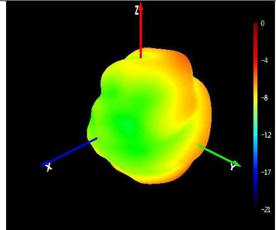
001# LTE antenna sample 3D orientation map (2350MHz)
