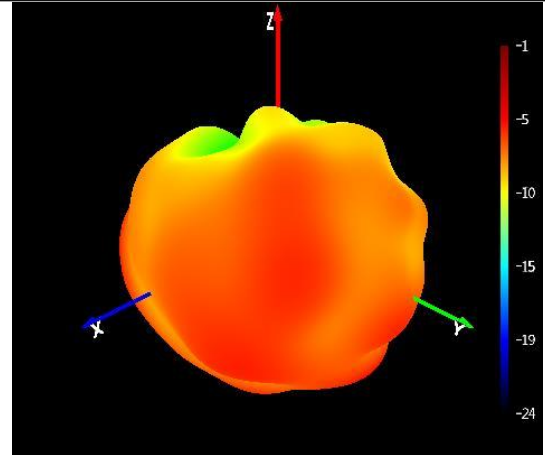
001# LTE antenna sample 3D orientation map (1860MHz)
