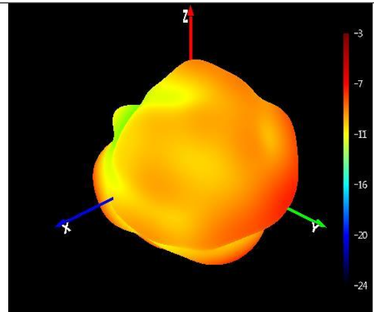
001# LTE antenna sample 3D orientation map (2060MHz)
