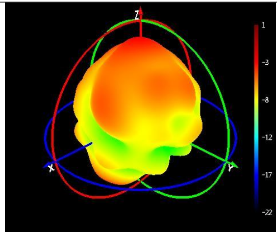
001#GNSS antenna sample 3D orientation map (1561.098MHz)
