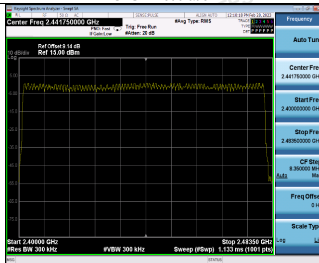
m/4DQPSK Modulation
