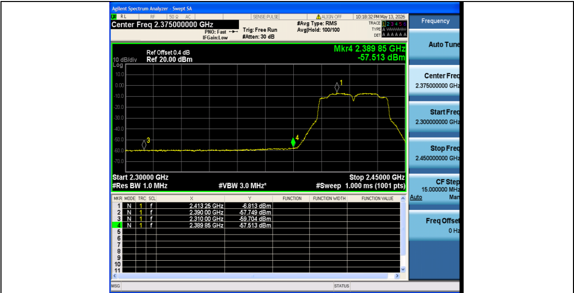
11N40SISO_Ant1_Low_2422_Peak
