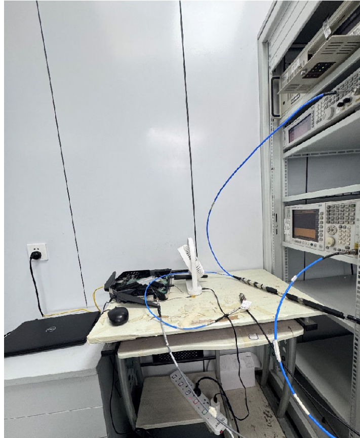
Picture 1 DFS Test Setup
