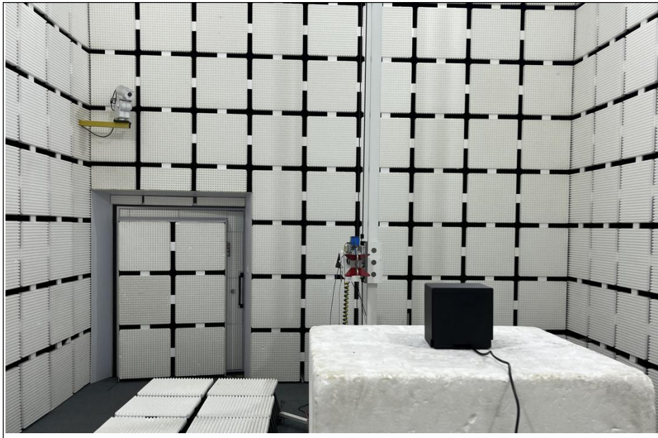
RADIATED EMISSION TEST (1GHz ~ 18GHz)
