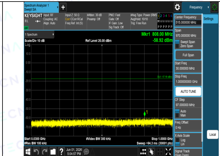
3DH5-Ant1-2402-30~1000-PASS
