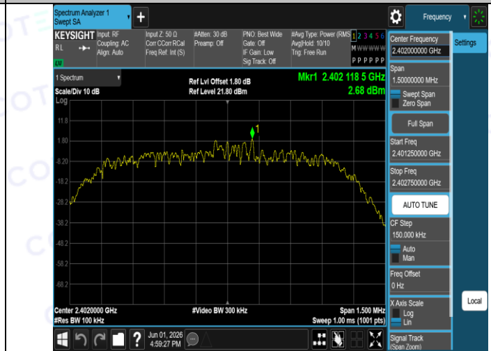
2DH5-Ant1-2402-0~Reference-PASS
