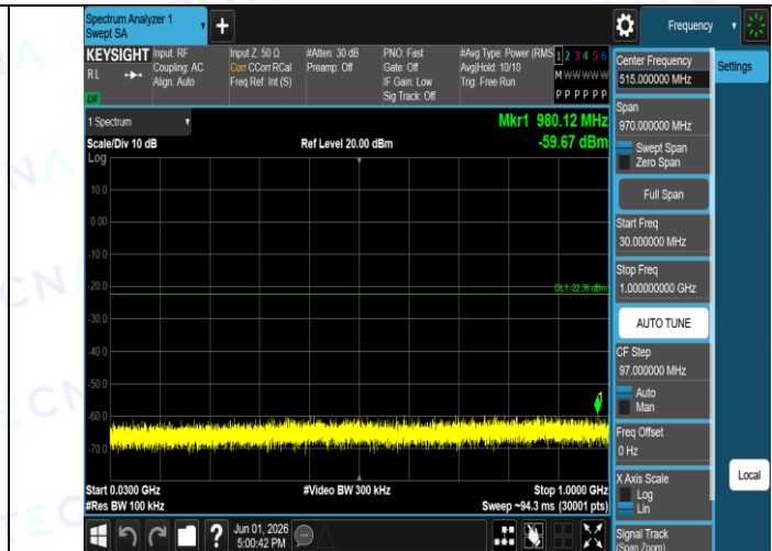
2DH5-Ant1-2441-30~1000-PASS
