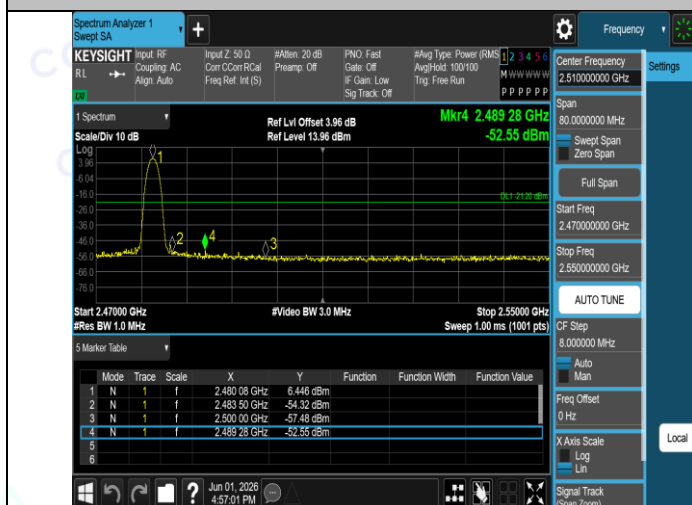
DH5-Ant1-2480-PASS
