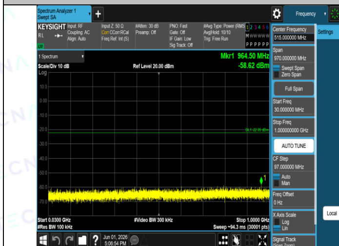
3DH5-Ant1-2441-30~1000-PASS
