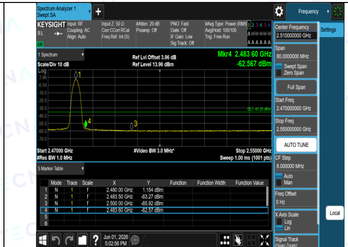
2DH5-Ant1-2480-PASS
