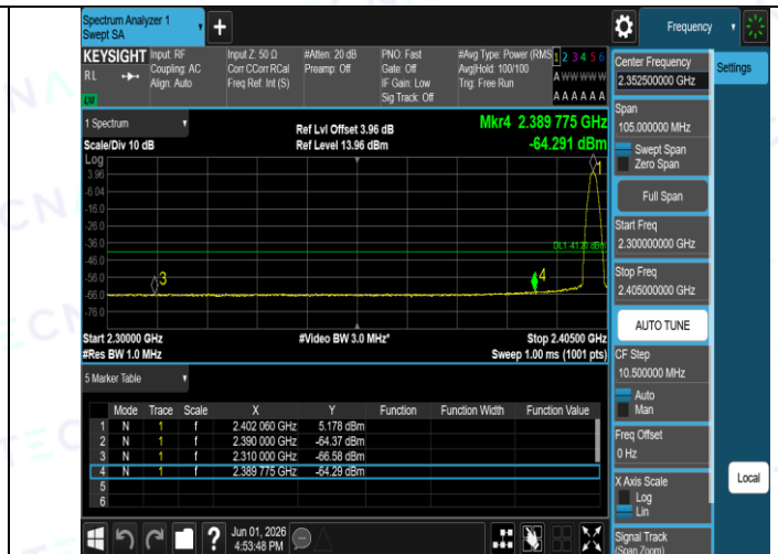
DH5-Ant1-2402-PASS
