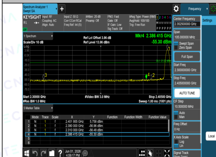
2DH5-Ant1-2402-PASS
