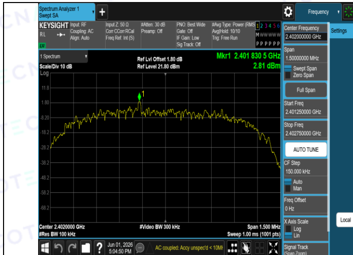
3DH5-Ant1-2402-0~Reference-PASS
