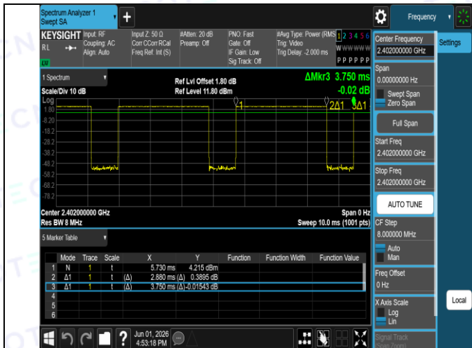
NTNV-DH5-Ant1-2402
