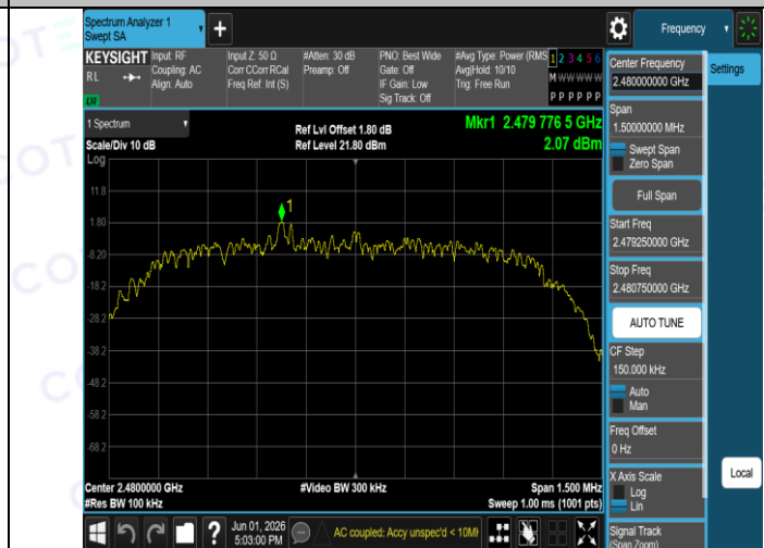
2DH5-Ant1-2480-0~Reference-PASS
