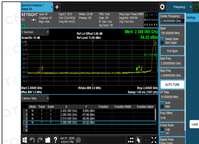
DH5-Ant1-2402-PASS
