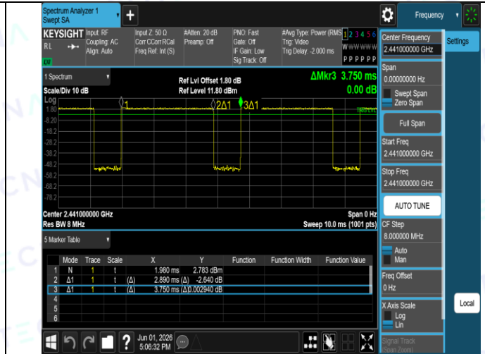
NTNV-3DH5-Ant1-2441
