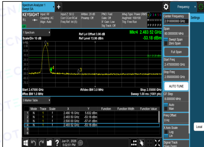
2DH5-Ant1-2480-PASS
