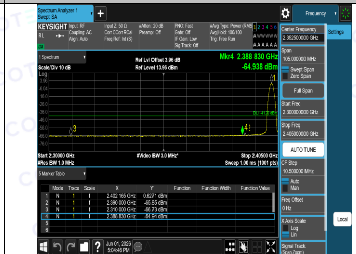
3DH5-Ant1-2402-PASS
