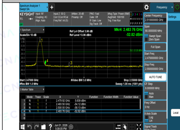
3DH5-Ant1-2480-PASS
