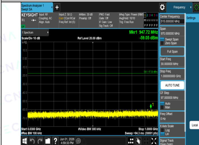
2DH5-Ant1-2402-30~1000-PASS
