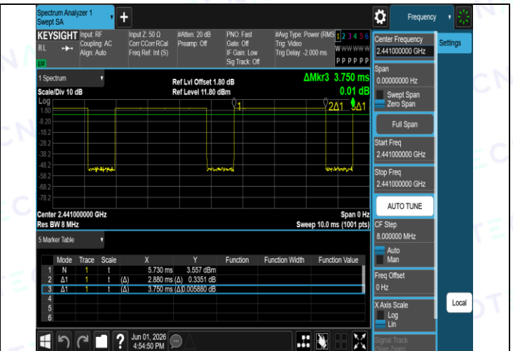
NTNV-DH5-Ant1-2441
