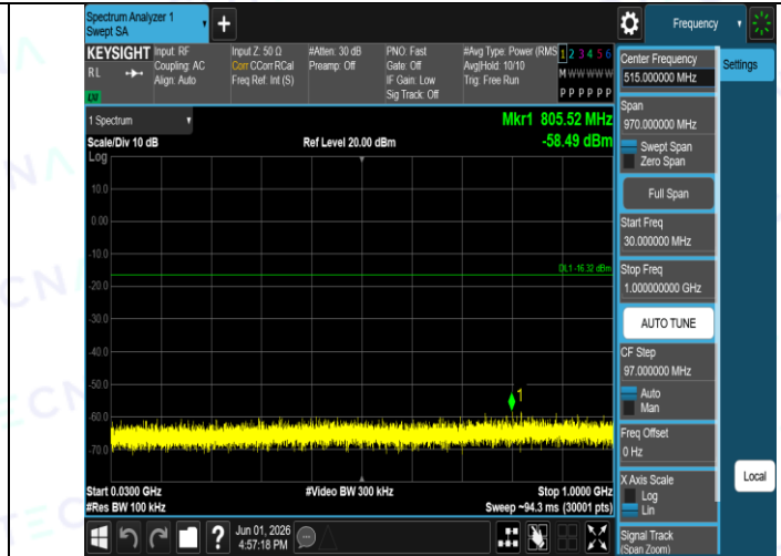
DH5-Ant1-2480-30~1000-PASS
