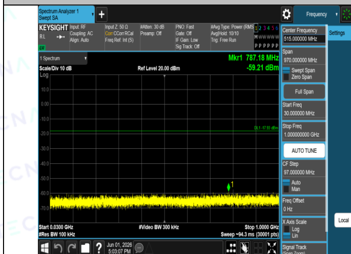
2DH5-Ant1-2480-30~1000-PASS
