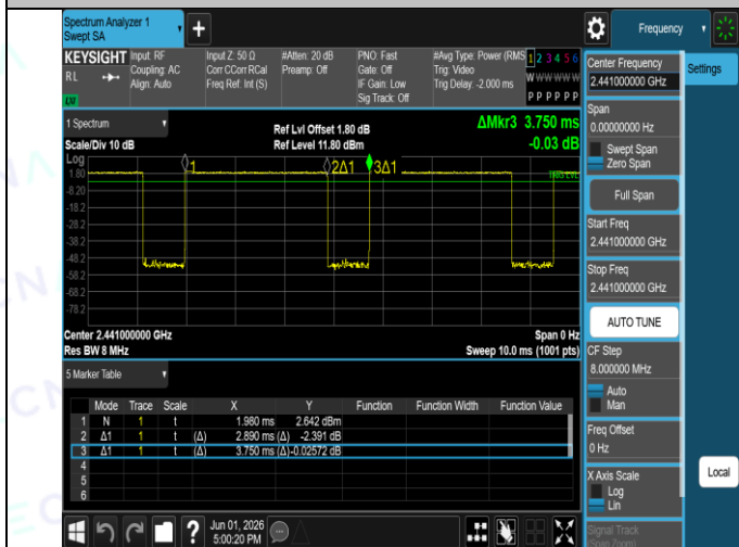
NTNV-2DH5-Ant1-2441
