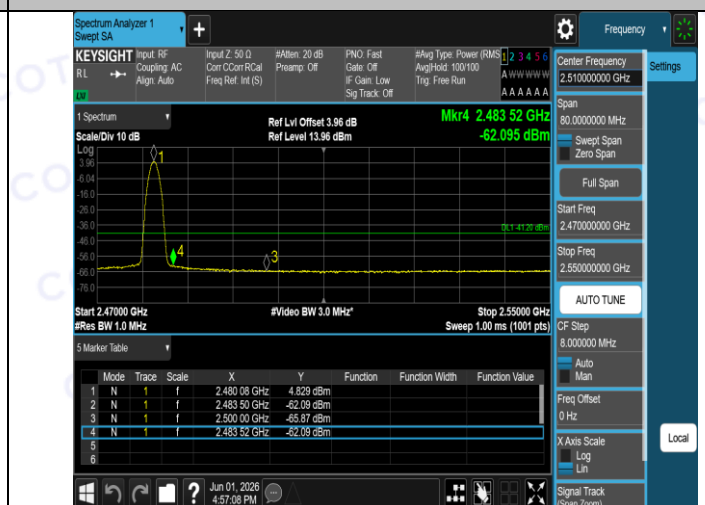
DH5-Ant1-2480-PASS
