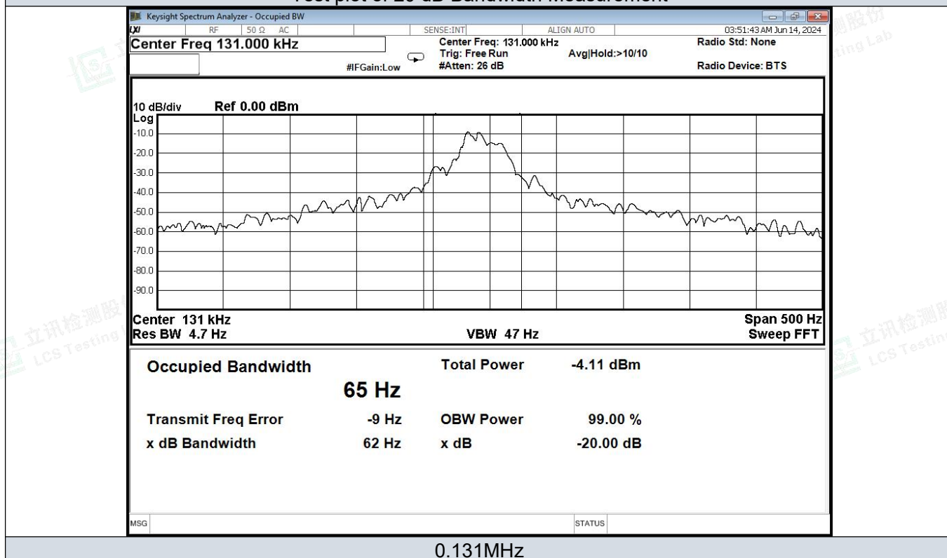
Test plot of 20 dB Bandwidth Measurement
