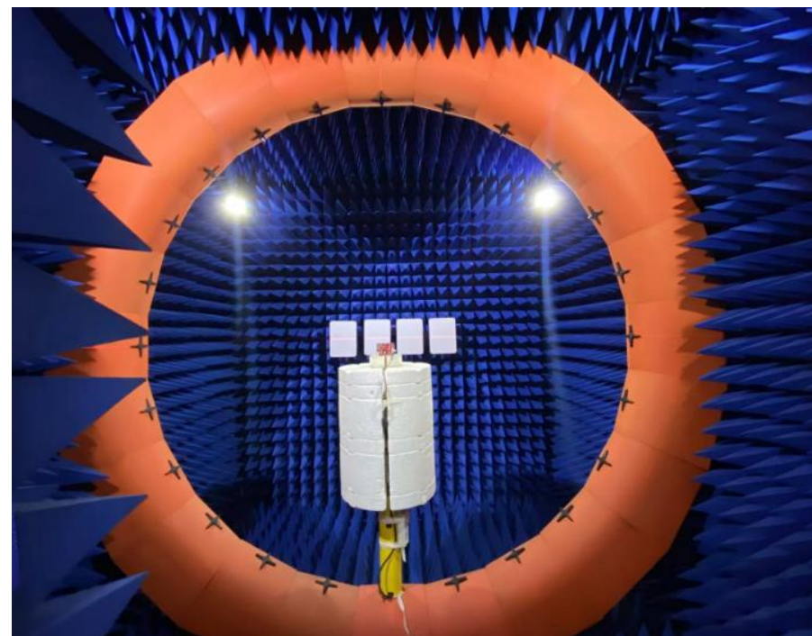
Testing 3D microwave darkroom(3m*3m*3m)
