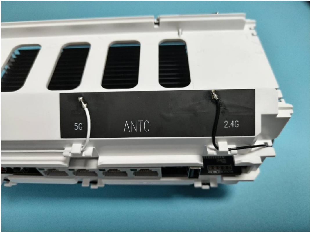
2.4G&5G ANT 0
