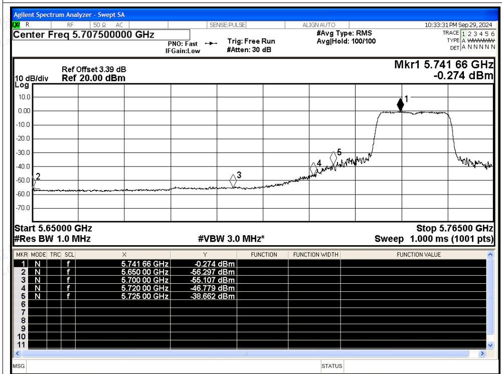
Restrict Band NVNT n20 5745MHz Ant1 Average
