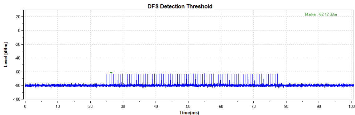
Radar Singal 1
