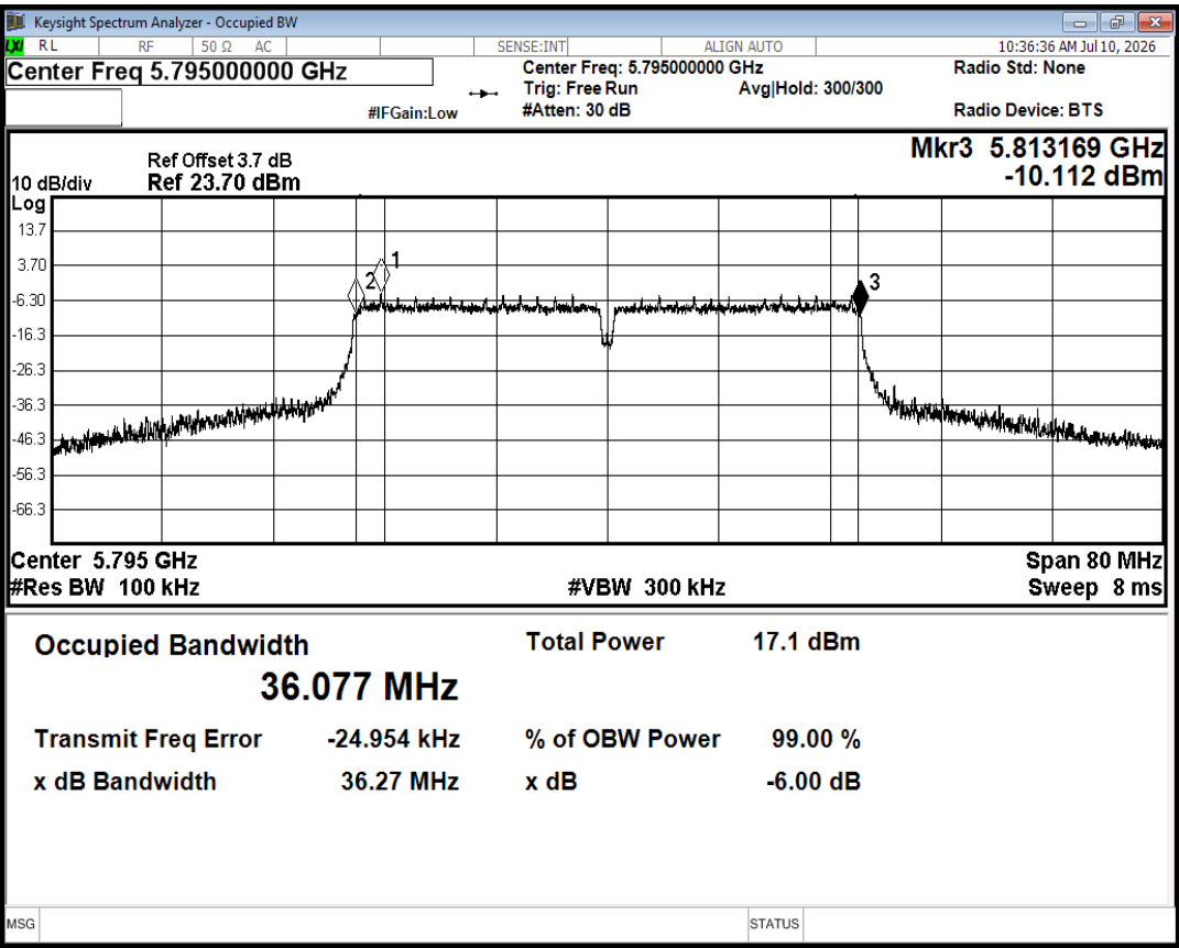
-6dB Bandwidth NVNT n40 5795MHz Ant2
