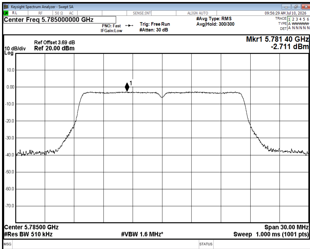
PSD NVNT a 5785MHz Ant2
