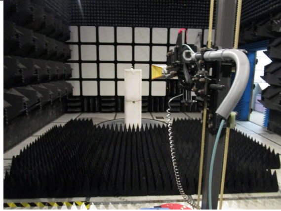
Above 1 GHz Setup
