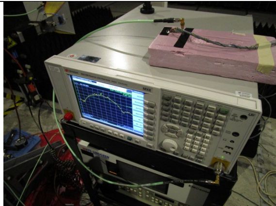
Conducted Setup
