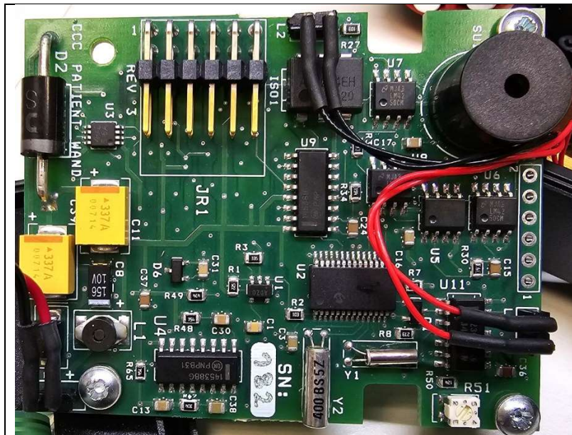
Patient Controller Internal Photo, Front of PCBA
