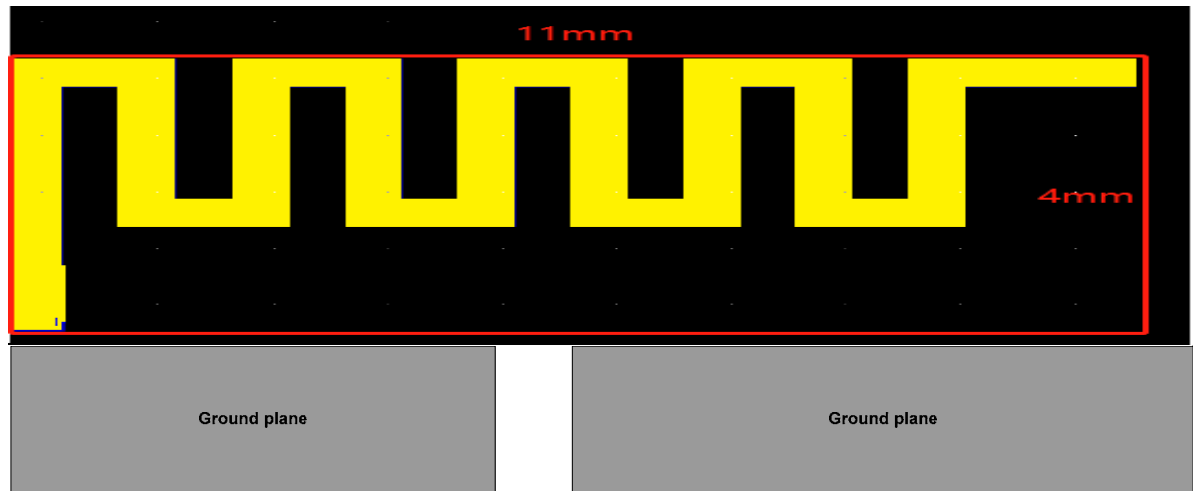
Figure 1. IFA Dimensions
