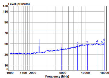
11b_TX_CH_06_Vertical-Peak
