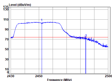
11n_HT(40M)_TX_CH_09_Horizontal-Peak
