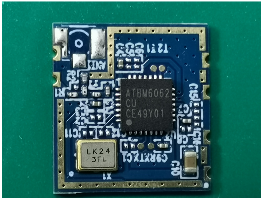
Model: ATBM6062-CT
