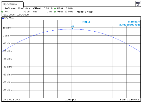
BLE_1M_Low_Channel
