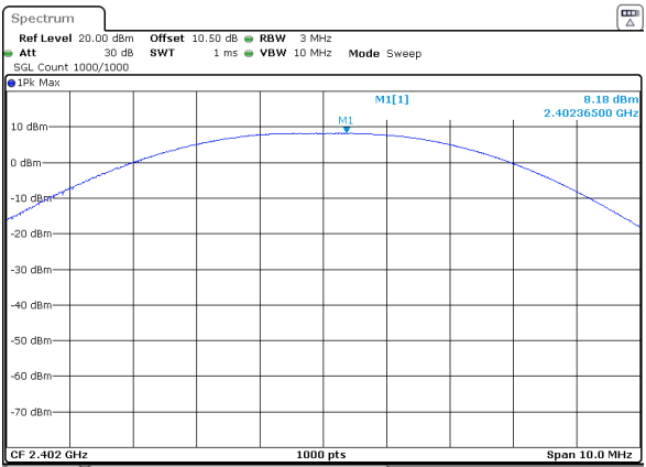
BLE_2M_Low_Channel
