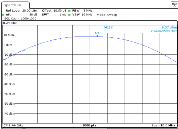
BLE_2M_Middle_Channel
