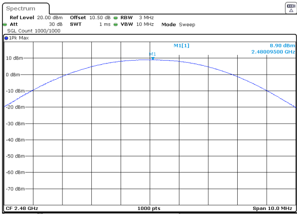
BLE_1M_High_Channel
