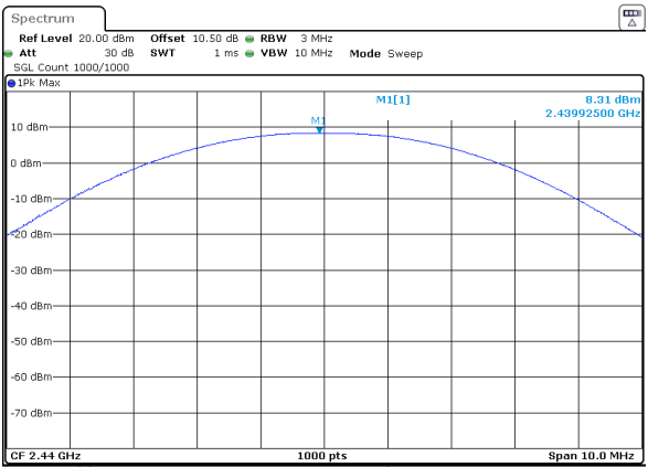
BLE_1M_Middle_Channel
