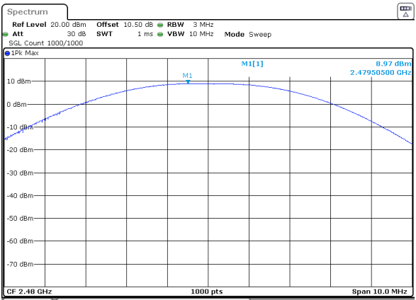
BLE_2M_High_Channel
