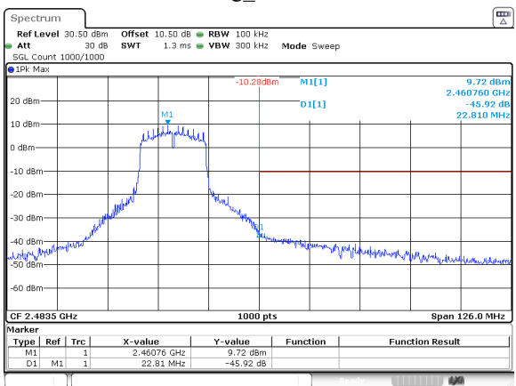
802.11g_2462MHz
