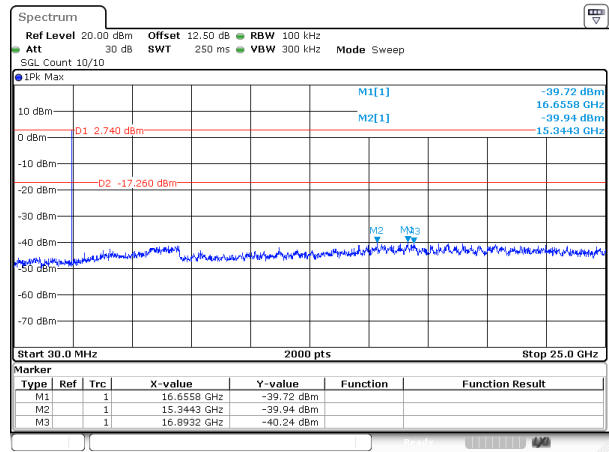
BLE_2M_High_Channel
