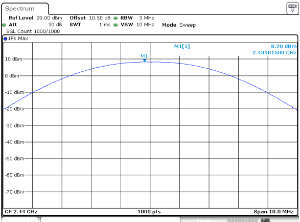
BLE_1M_Middle_Channel
