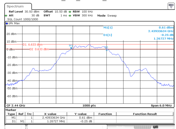
BLE_2M_Middle_Channel
