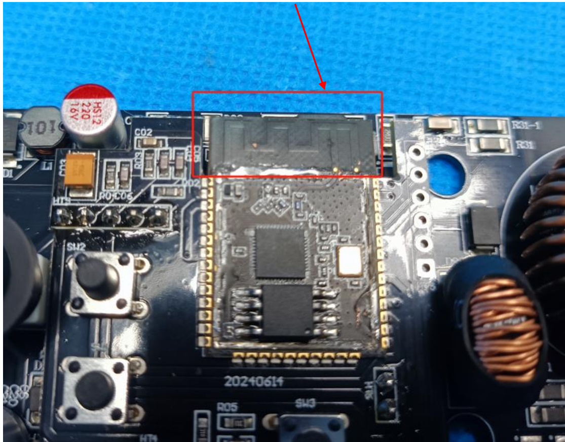
RF antenna
