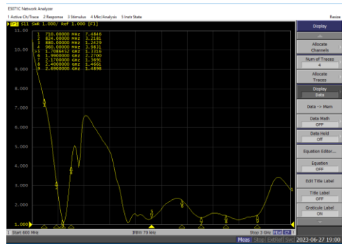
A101 WIFI 2 VSWR/Return Loss
