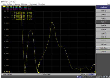
A101 WIFI 1 VSWR/Return Loss
