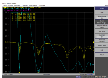
A101 WIFI 2 VSWR/Return Loss
