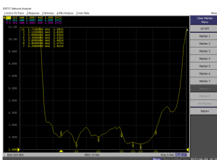
A101 ANT3 VSWR/Return Loss
