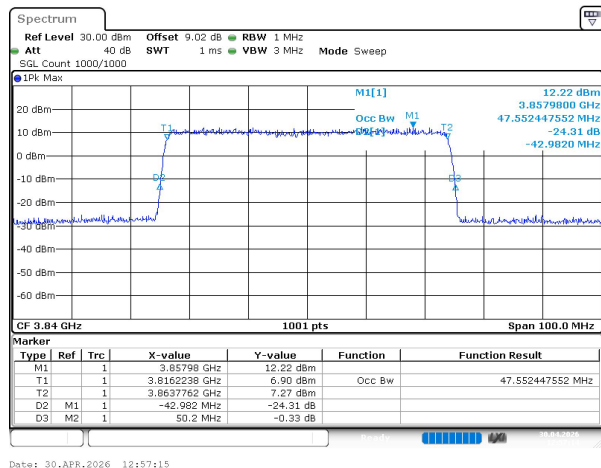
n77(3700-3980) SCS=30kHz CP_64QAM BW=50MHz Channel=656000 RB=133@0
