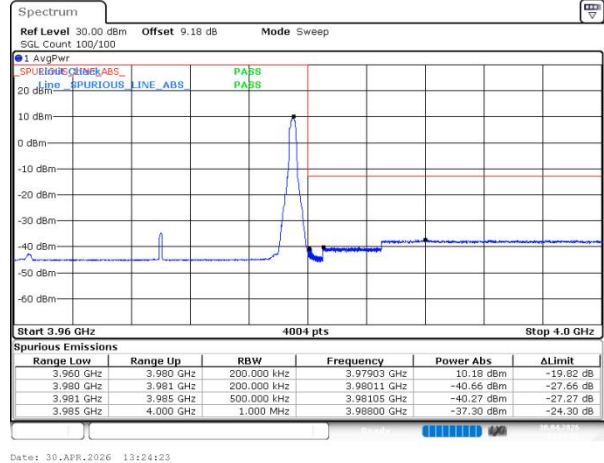
n77(3700-3980) SCS=30kHz DFT_64QAM BW=20MHz HighChannel=664666 RB=1@50
