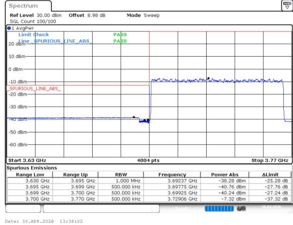
n77(3700-3980) SCS=30kHz DFT_64QAM BW=70MHz LowChannel=649000 RB=180@0
