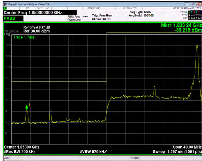
Band2 16QAM BW=20MHz Channel=18700 RB Size=100 Position=#0 Extended
