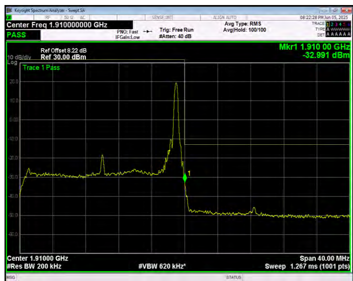
Band2 16QAM BW=20MHz Channel=19100 RB Size=100 Position=#0 Extended
