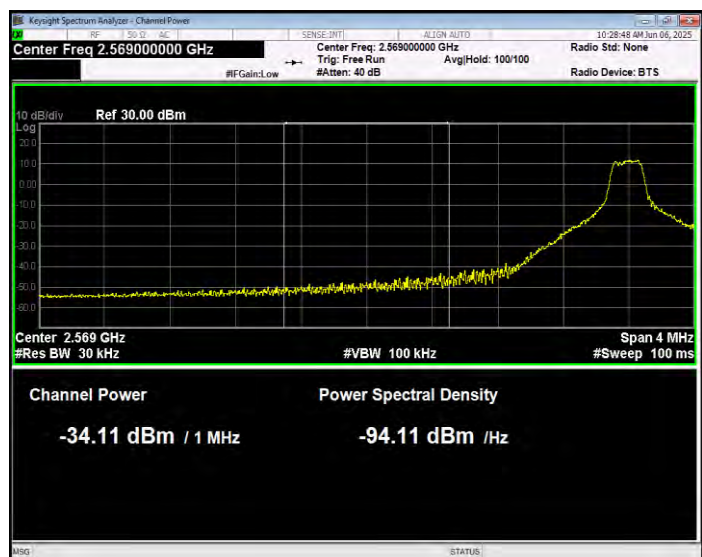
Band38 QPSK BW=10MHz Channel=37800 RB Size=1 Position=#0 Normal
