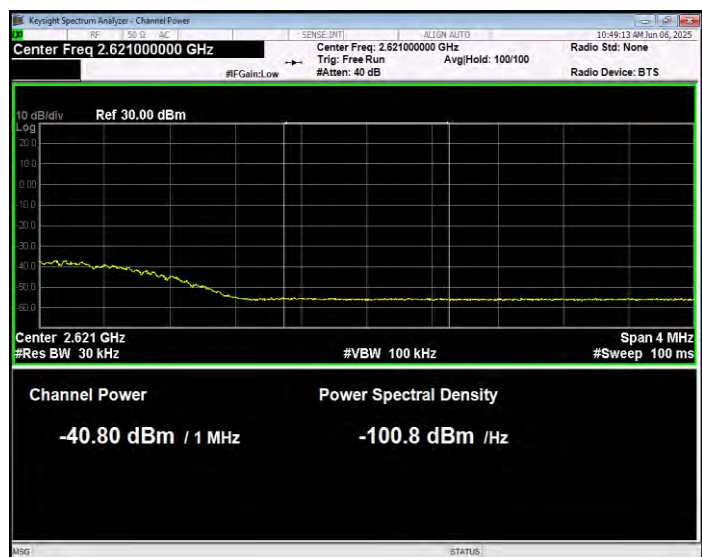
Band38 QPSK BW=15MHz Channel=38175 RB Size=1 Position=#0 Normal
