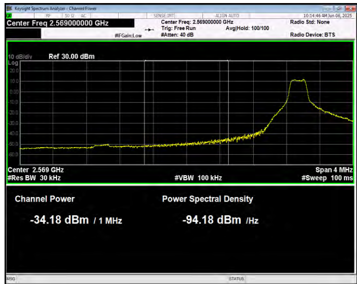
Band38 QPSK BW=5MHz Channel=37775 RB Size=1 Position=#0 Normal
