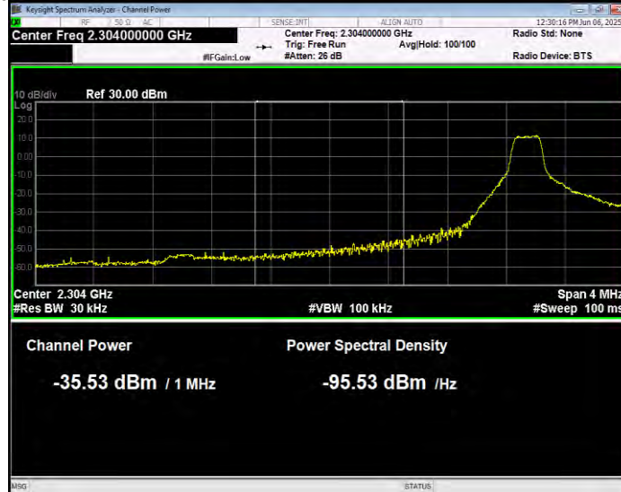
Band40(2305-2315) QPSK BW=5MHz Channel=38725 RB Size=1 Position=#0 Normal
