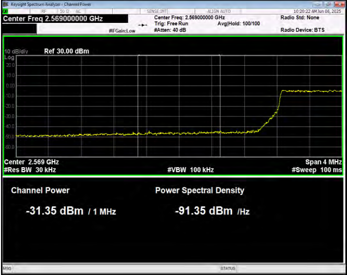
Band38 16QAM BW=5MHz Channel=37775 RB Size=25 Position=#0 Normal
