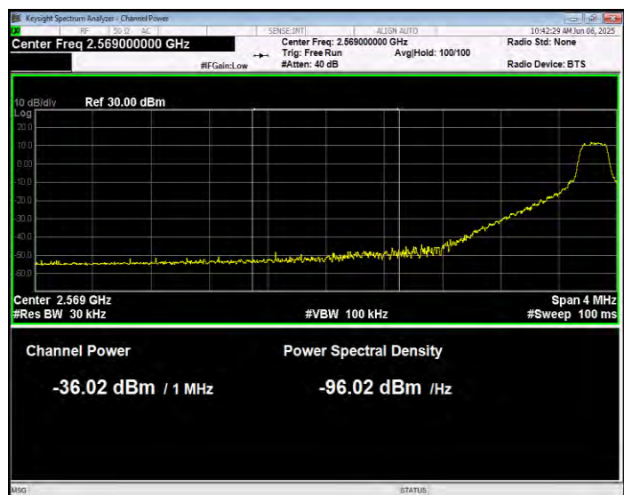
Band38 QPSK BW=15MHz Channel=37825 RB Size=1 Position=#0 Normal
