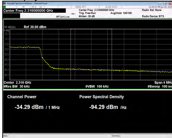
Band40(2305-2315) 16QAM BW=5MHz Channel=38775 RB Size=25 Position=#0 Normal
