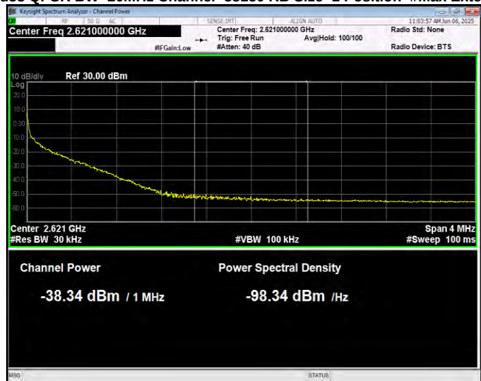
Band38 QPSK BW=20MHz Channel=38150 RB Size=1 Position=#Max Normal
