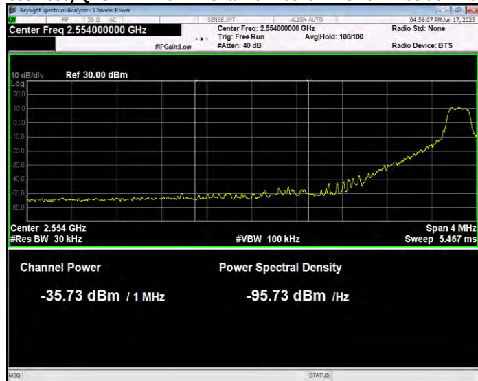
Band41(2555-2655) QPSK BW=15MHz Channel=40315 RB Size=1 Position=#0 Normal
