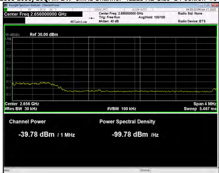
Band41(2555-2655) 16QAM BW=5MHz Channel=41215 RB Size=1 Position=#0 Normal
