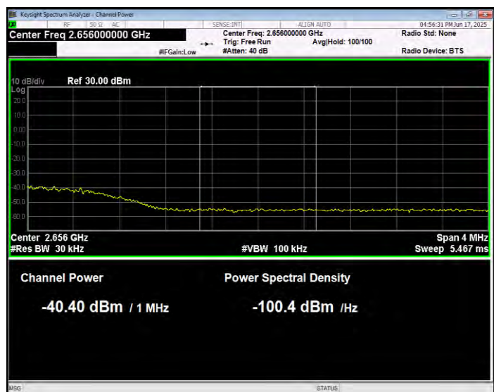
Band41(2555-2655) 16QAM BW=15MHz Channel=41165 RB Size=1 Position=#0 Normal
