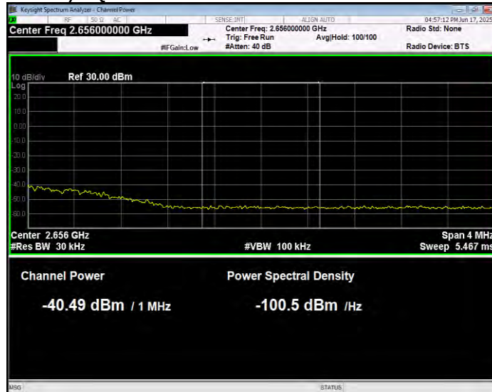
Band41(2555-2655) 16QAM BW=20MHz Channel=41140 RB Size=1 Position=#0 Normal
