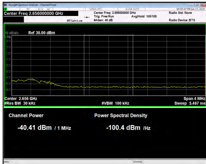
Band41(2555-2655) QPSK BW=10MHz Channel=41190 RB Size=1 Position=#0 Normal
