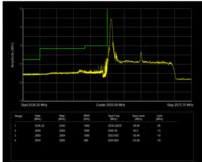
Band41(2555-2655) QPSK BW=15MHz Channel=41165 RB Size=1 Position=#0 Extended
