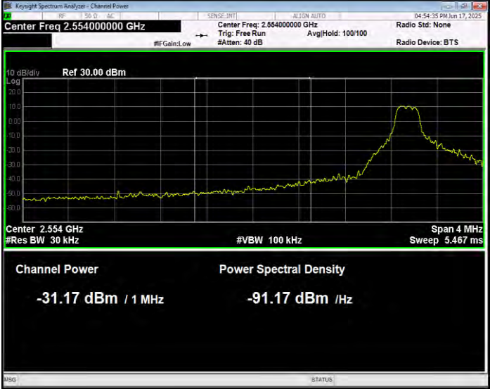
Band41(2555-2655) QPSK BW=5MHz Channel=40265 RB Size=1 Position=#0 Normal
