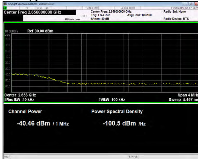
Band41(2555-2655) QPSK BW=15MHz Channel=41165 RB Size=1 Position=#0 Normal
