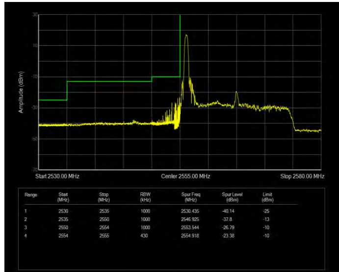
Band41(2555-2655) 16QAM BW=20MHz Channel=41140 RB Size=1 Position=#0 Extended
