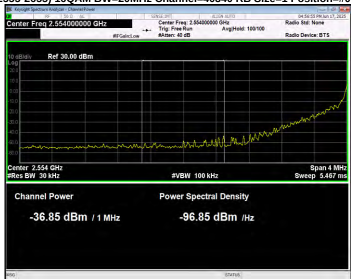
Band41(2555-2655) 16QAM BW=20MHz Channel=40340 RB Size=1 Position=#0 Normal
