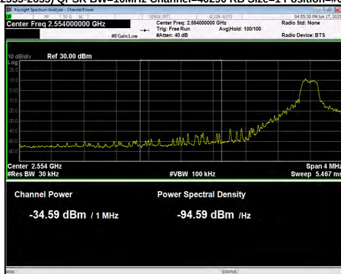
Band41(2555-2655) QPSK BW=10MHz Channel=40290 RB Size=1 Position=#0 Normal
