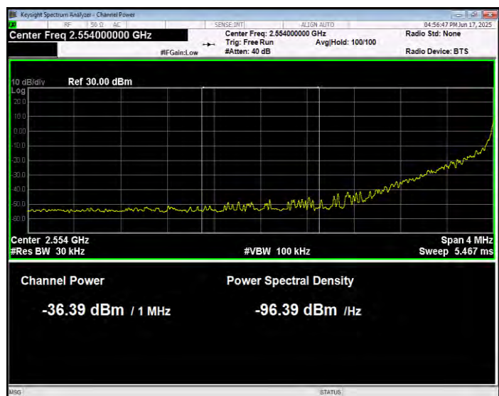
Band41(2555-2655) QPSK BW=20MHz Channel=40340 RB Size=1 Position=#0 Normal
