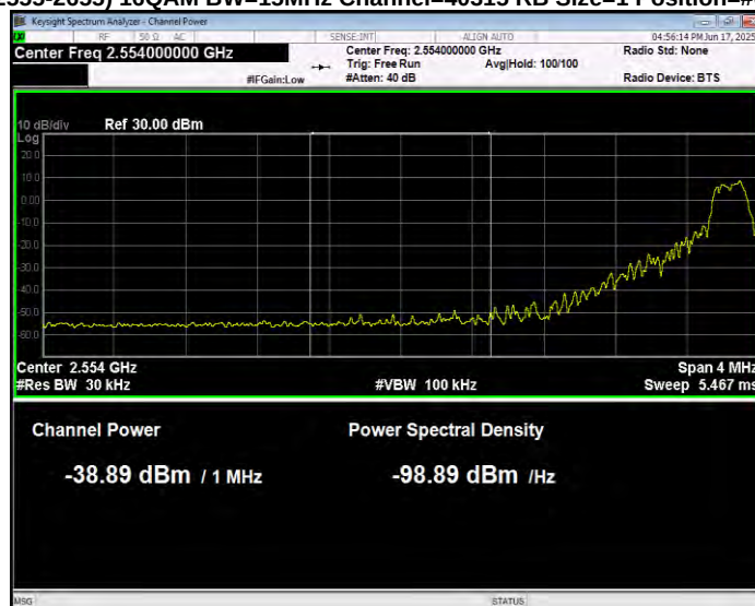
Band41(2555-2655) 16QAM BW=15MHz Channel=40315 RB Size=1 Position=#0 Normal
