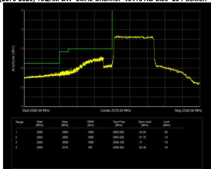
Band41(2570-2620) 16QAM BW=5MHz Channel=40415 RB Size=25 Position=#0 Normal
