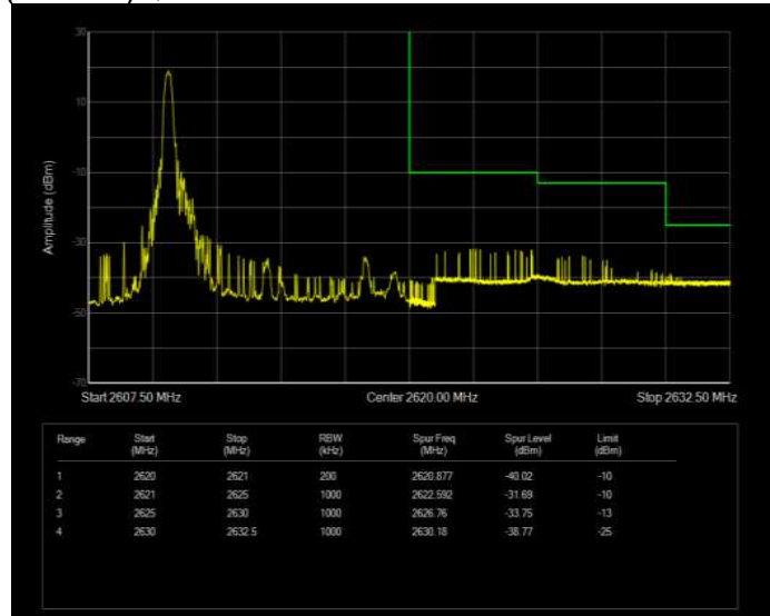
Band41(2570-2620) QPSK BW=10MHz Channel=40840 RB Size=1 Position=#Max Normal
