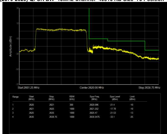
Band41(2570-2620) QPSK BW=15MHz Channel=40815 RB Size=75 Position=#0 Normal
