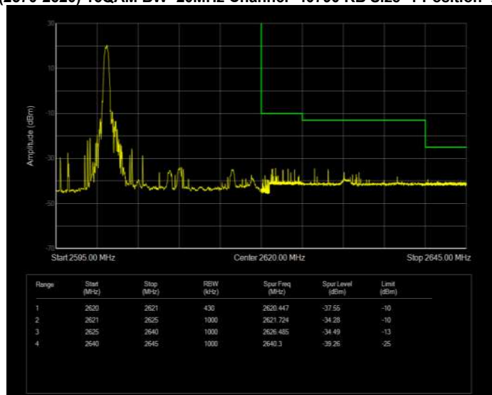
Band41(2570-2620) 16QAM BW=20MHz Channel=40790 RB Size=1 Position=#Max Normal
