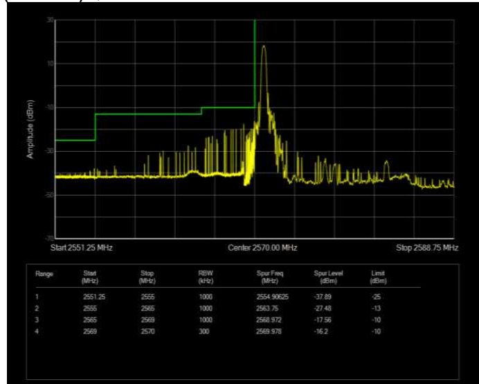
Band41(2570-2620) QPSK BW=15MHz Channel=40465 RB Size=1 Position=#Max Normal
