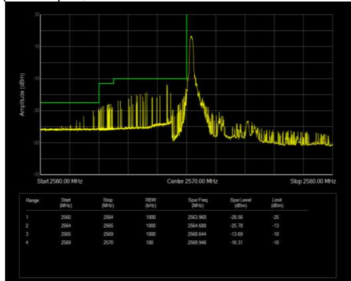
Band41(2570-2620) 16QAM BW=5MHz Channel=40415 RB Size=1 Position=#Max Normal
