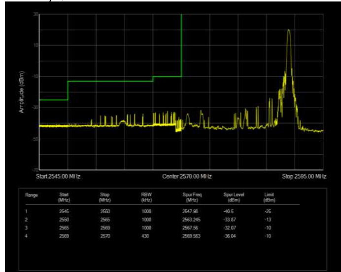
Band41(2570-2620) QPSK BW=20MHz Channel=40490 RB Size=100 Position=#0 Normal
