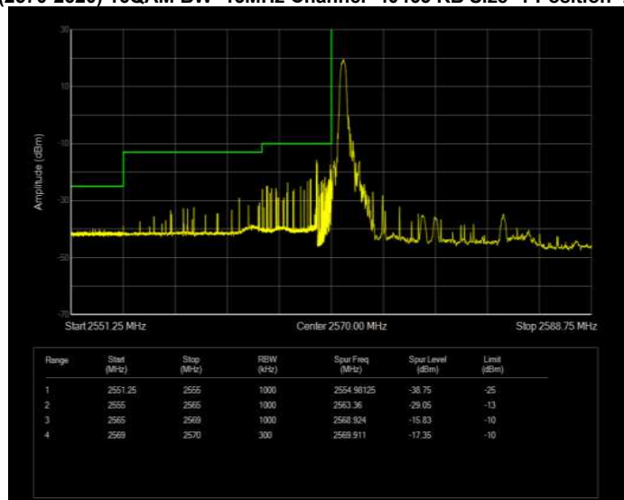
Band41(2570-2620) 16QAM BW=15MHz Channel=40465 RB Size=1 Position=#Max Normal
