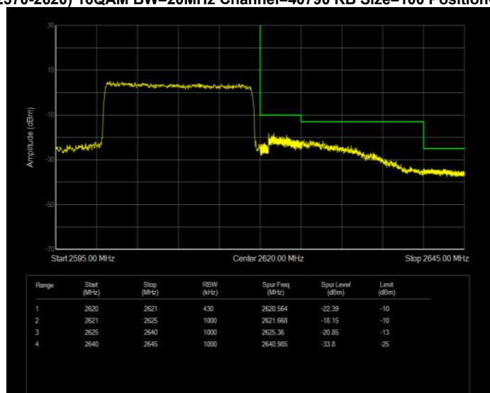
Band41(2570-2620) 16QAM BW=20MHz Channel=40790 RB Size=100 Position=#0 Normal
