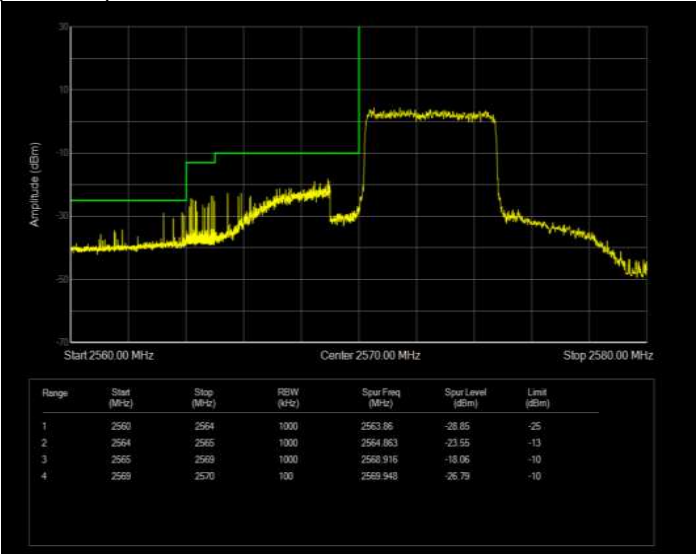
Band41(2570-2620) QPSK BW=5MHz Channel=40415 RB Size=25 Position=#0 Normal
