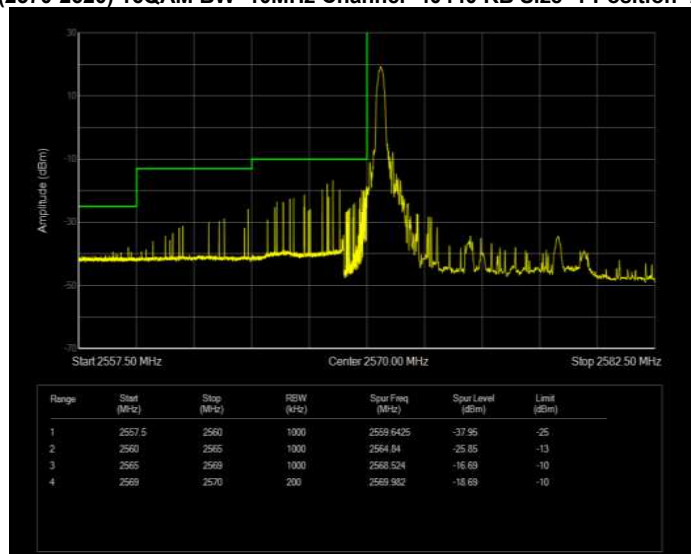
Band41(2570-2620) 16QAM BW=10MHz Channel=40440 RB Size=1 Position=#Max Normal
