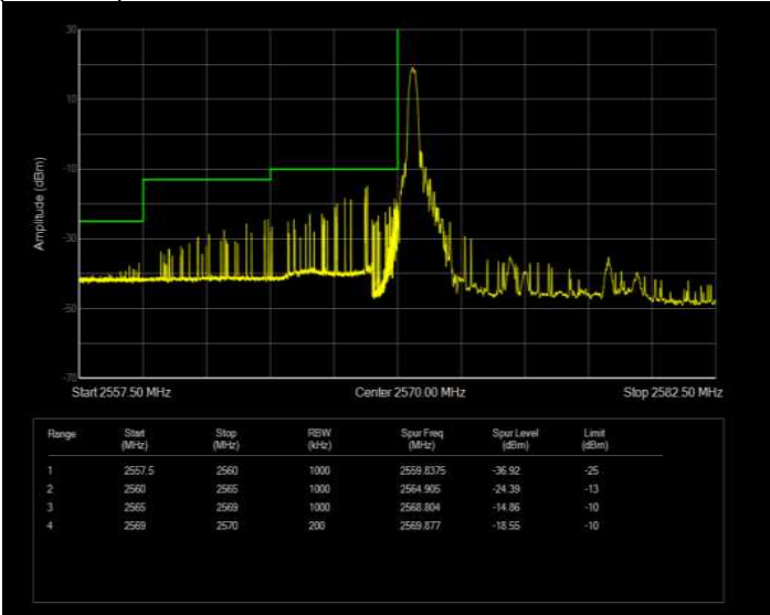
Band41(2570-2620) QPSK BW=10MHz Channel=40440 RB Size=1 Position=#Max Normal
