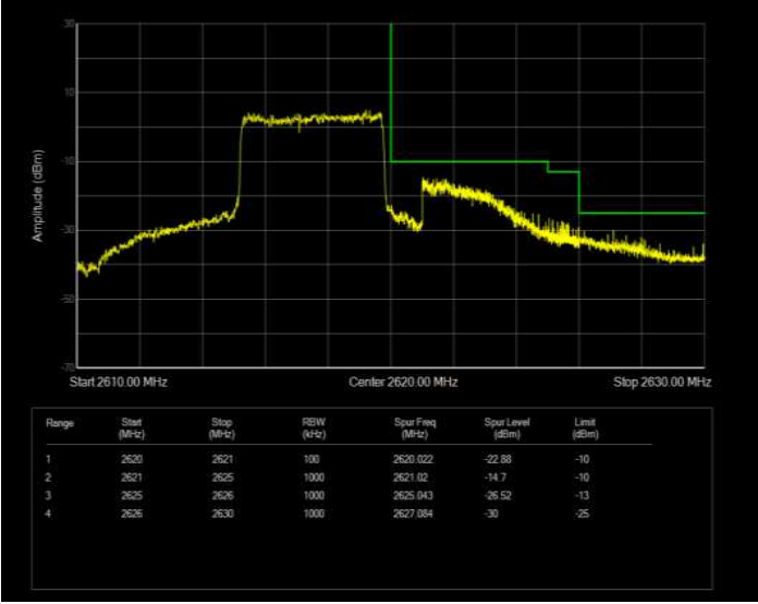
Band41(2570-2620) QPSK BW=5MHz Channel=40865 RB Size=25 Position=#0 Normal
