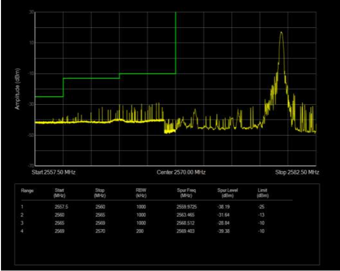
Band41(2570-2620) QPSK BW=10MHz Channel=40440 RB Size=50 Position=#0 Normal
