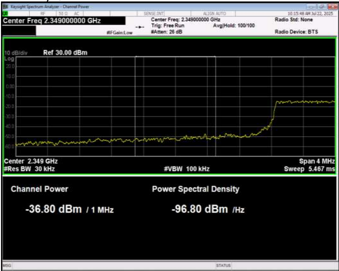
Band40(2350-2360) QPSK BW=5MHz Channel=39175 RB Size=25 Position=#0 Normal
