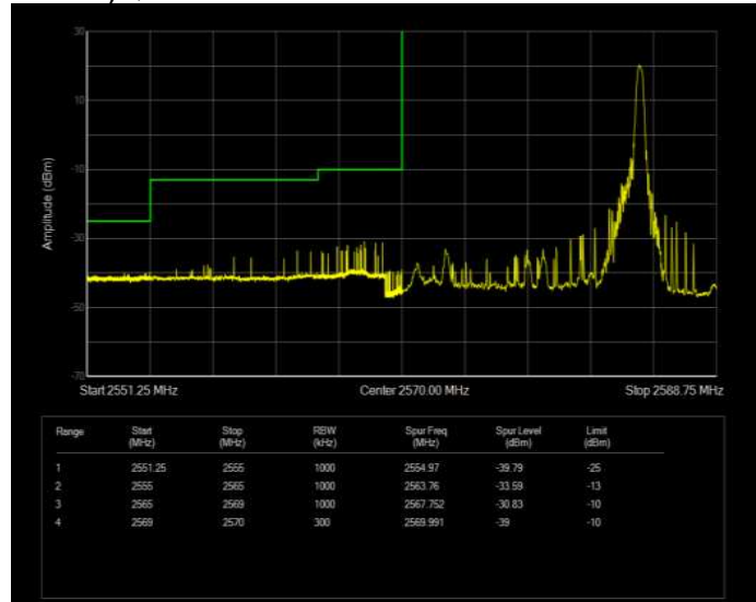
Band41(2570-2620) QPSK BW=15MHz Channel=40465 RB Size=75 Position=#0 Normal
