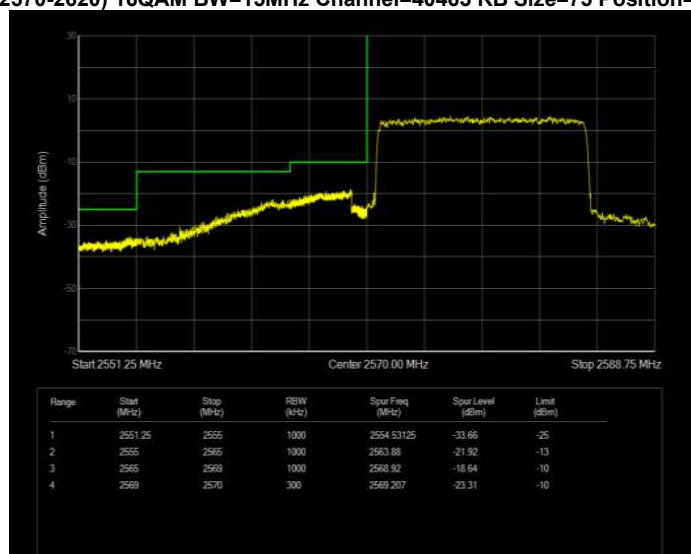
Band41(2570-2620) 16QAM BW=15MHz Channel=40465 RB Size=75 Position=#0 Normal
