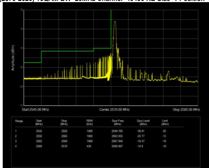
Band41(2570-2620) 16QAM BW=20MHz Channel=40490 RB Size=1 Position=#Max Normal
