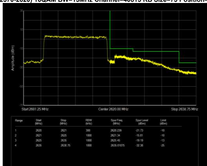
Band41(2570-2620) 16QAM BW=15MHz Channel=40815 RB Size=75 Position=#0 Normal
