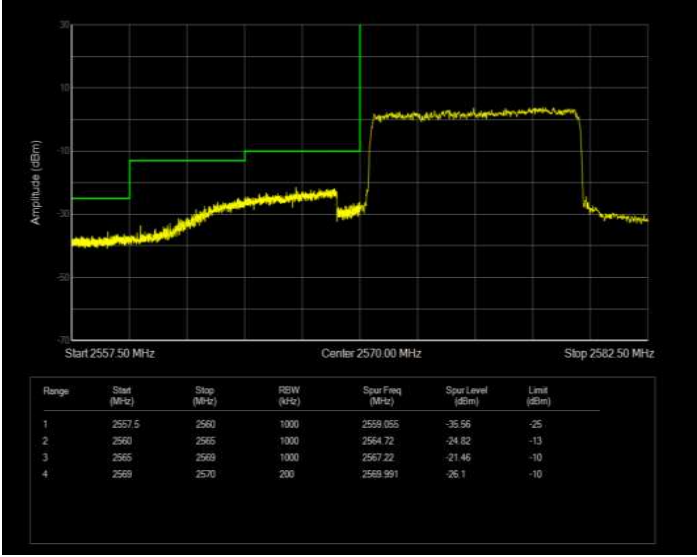
Band41(2570-2620) QPSK BW=10MHz Channel=40440 RB Size=50 Position=#0 Normal
