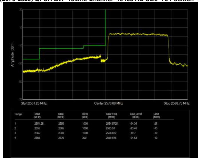
Band41(2570-2620) QPSK BW=15MHz Channel=40465 RB Size=75 Position=#0 Normal
