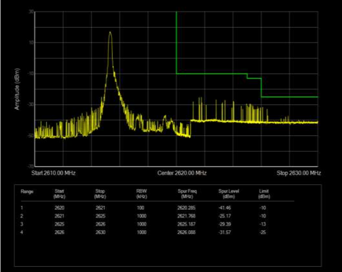
Band41(2570-2620) QPSK BW=5MHz Channel=40865 RB Size=1 Position=#Max Normal
