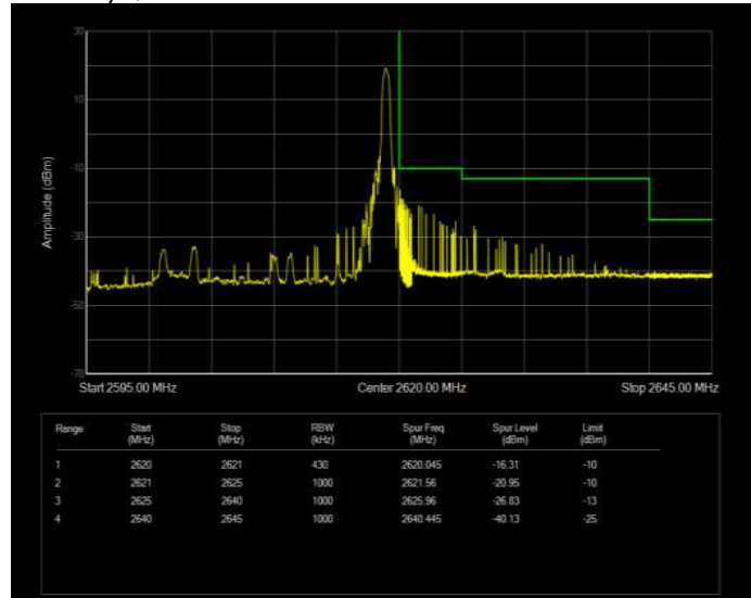
Band41(2570-2620) QPSK BW=20MHz Channel=40790 RB Size=100 Position=#0 Normal
