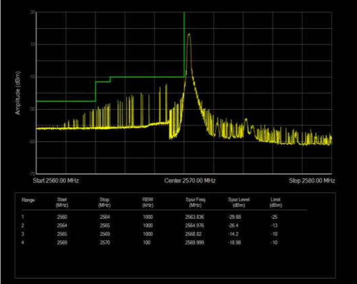
Band41(2570-2620) QPSK BW=5MHz Channel=40415 RB Size=1 Position=#Max Normal
