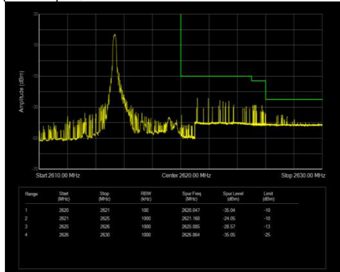
Band41(2570-2620) 16QAM BW=5MHz Channel=40865 RB Size=1 Position=#Max Normal
