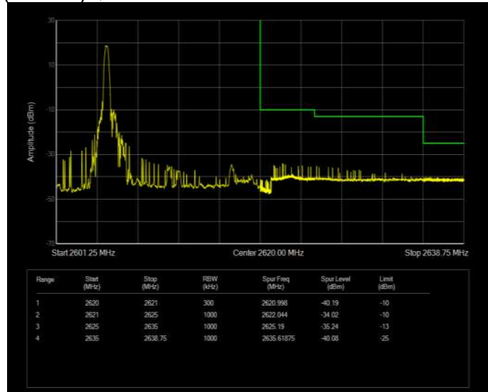
Band41(2570-2620) QPSK BW=15MHz Channel=40815 RB Size=1 Position=#Max Normal
