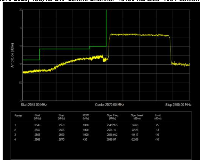
Band41(2570-2620) 16QAM BW=20MHz Channel=40490 RB Size=100 Position=#0 Normal
