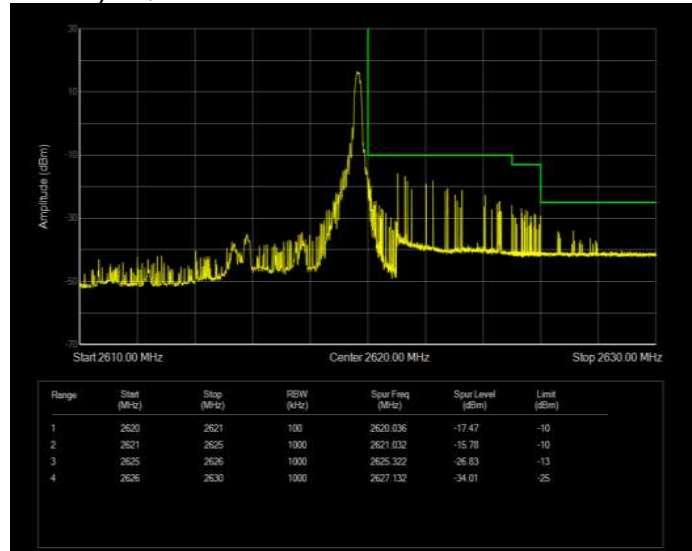
Band41(2570-2620) 16QAM BW=5MHz Channel=40865 RB Size=25 Position=#0 Normal
