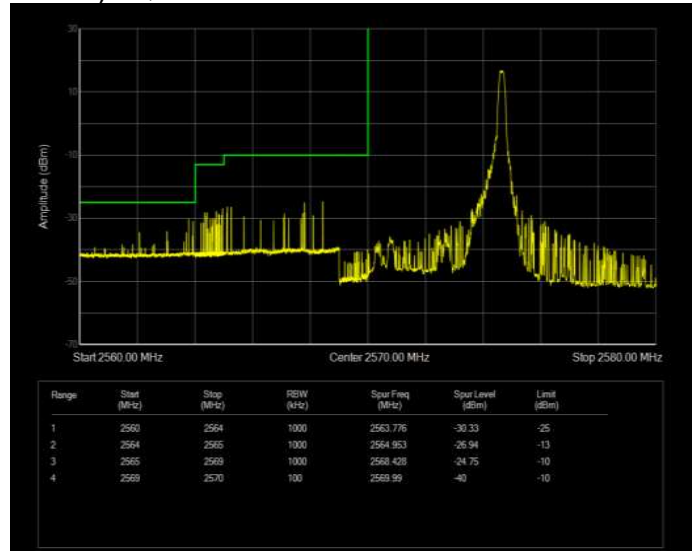
Band41(2570-2620) 16QAM BW=5MHz Channel=40415 RB Size=25 Position=#0 Normal
