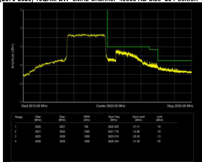
Band41(2570-2620) 16QAM BW=5MHz Channel=40865 RB Size=25 Position=#0 Normal
