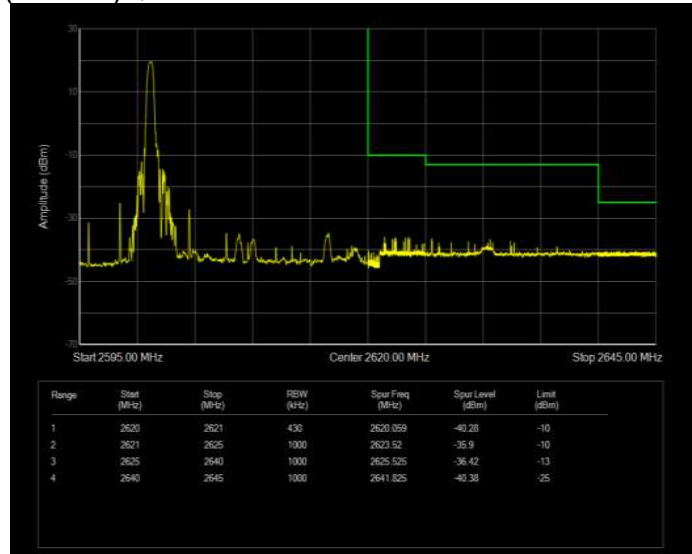
Band41(2570-2620) QPSK BW=20MHz Channel=40790 RB Size=1 Position=#Max Normal
