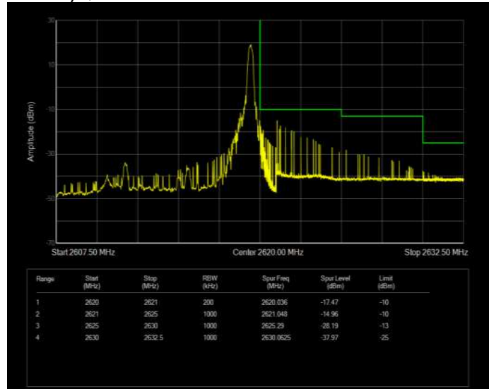
Band41(2570-2620) QPSK BW=10MHz Channel=40840 RB Size=50 Position=#0 Normal
