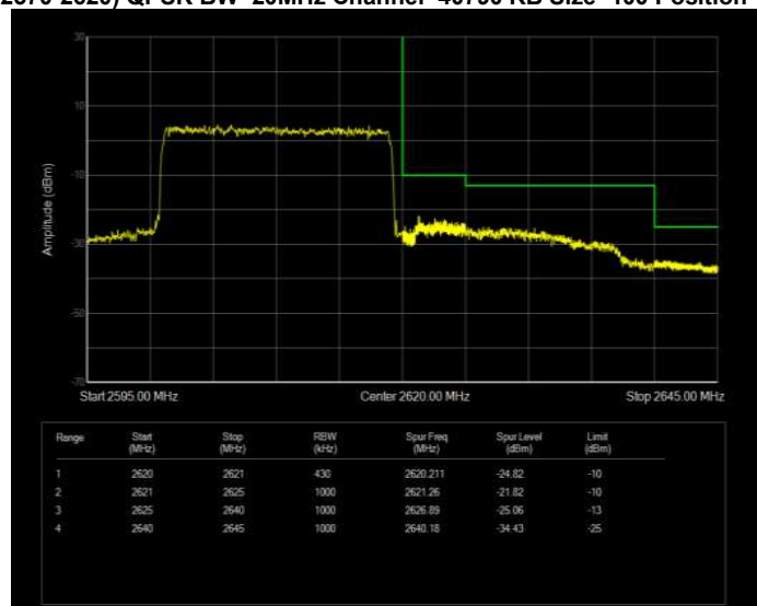
Band41(2570-2620) QPSK BW=20MHz Channel=40790 RB Size=100 Position=#0 Normal
