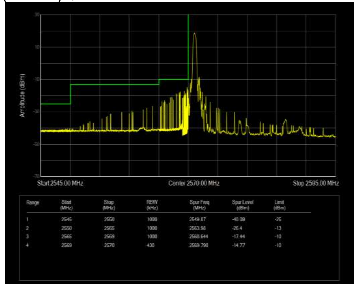
Band41(2570-2620) QPSK BW=20MHz Channel=40490 RB Size=1 Position=#Max Normal
