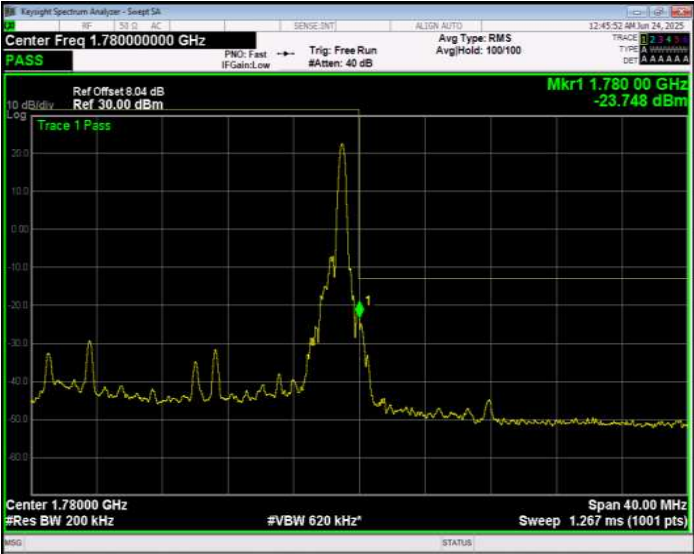
Band66 QPSK BW=20MHz Channel=132572 RB Size=100 Position=#0 Extended
