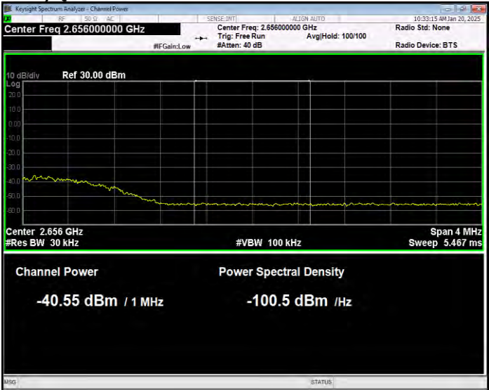
Band41(2555-2655) QPSK BW=15MHz Channel=41165 RB Size=1 Position=#0 Normal
