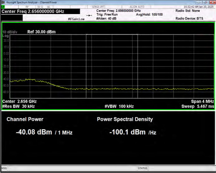
Band41(2555-2655) 16QAM BW=10MHz Channel=41190 RB Size=1 Position=#0 Extended
