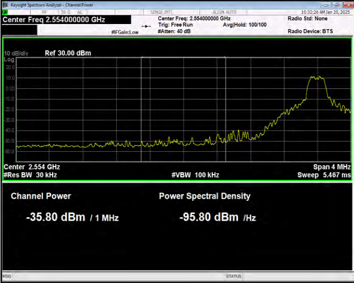
Band41(2555-2655) 16QAM BW=10MHz Channel=40290 RB Size=1 Position=#0 Normal
