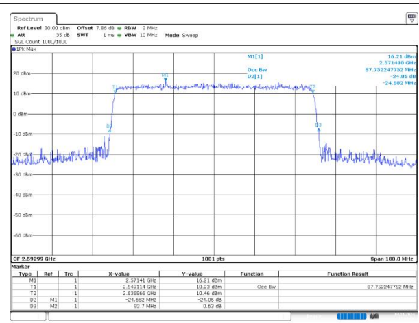
n41 SCS=30kHz CP_256QAM BW=80MHz Channel=518598 RB=217@0
