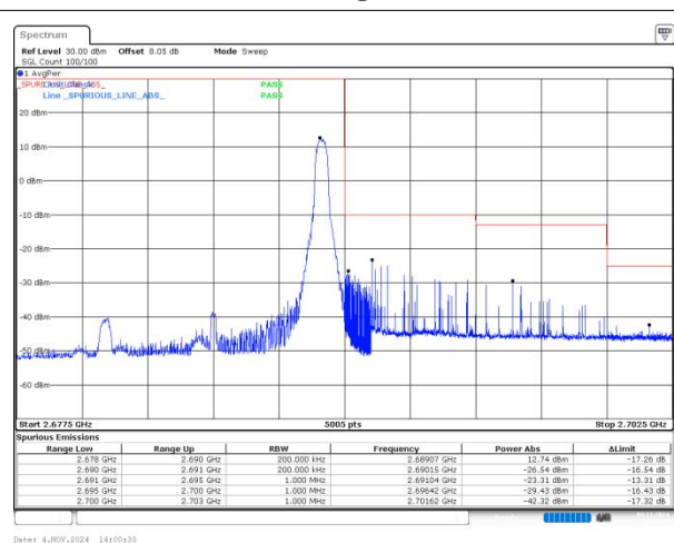
n41 SCS=30kHz DFT_64QAM BW=10MHz HighChannel=537000 RB=1@23
