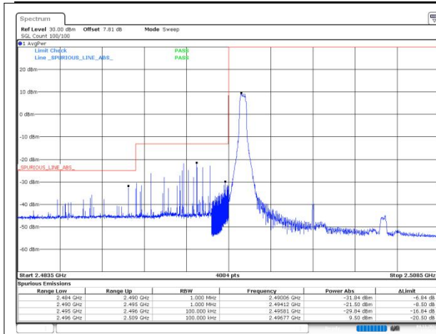
n41 SCS=30kHz DFT_64QAM BW=10MHz LowChannel=500202 RB=1@0
