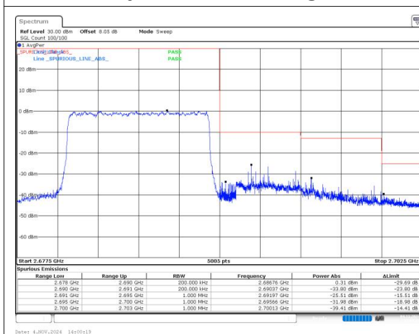
n41 SCS=30kHz DFT_16QAM BW=10MHz HighChannel=537000 RB=24@0
