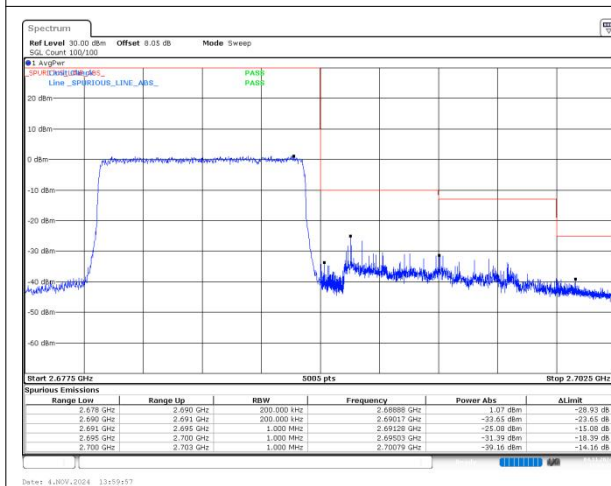
n41 SCS=30kHz DFT_QPSK BW=10MHz HighChannel=537000 RB=24@0
