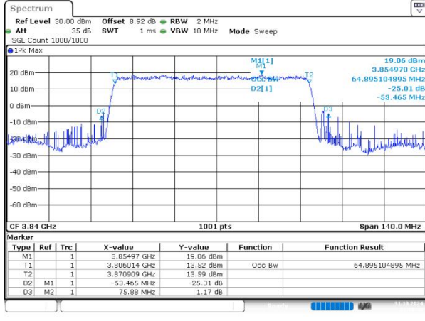
n77(3700-3980) SCS=30kHz DFT_BPSK BW=70MHz Channel=656000 RB=180@0
