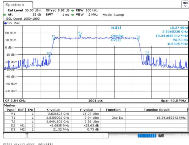
n77(3700-3980) SCS=30kHz CP_64QAM BW=20MHz Channel=656000 RB=51@0
