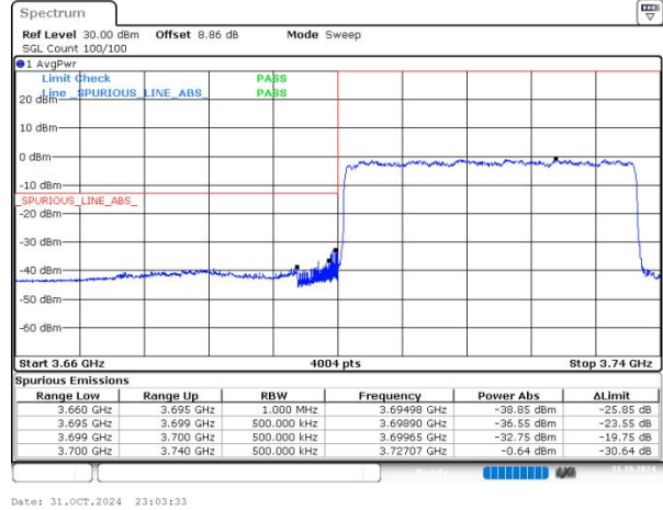
n77(3700-3980) SCS=30kHz DFT_BPSK BW=40MHz LowChannel=648000 RB=100@0
