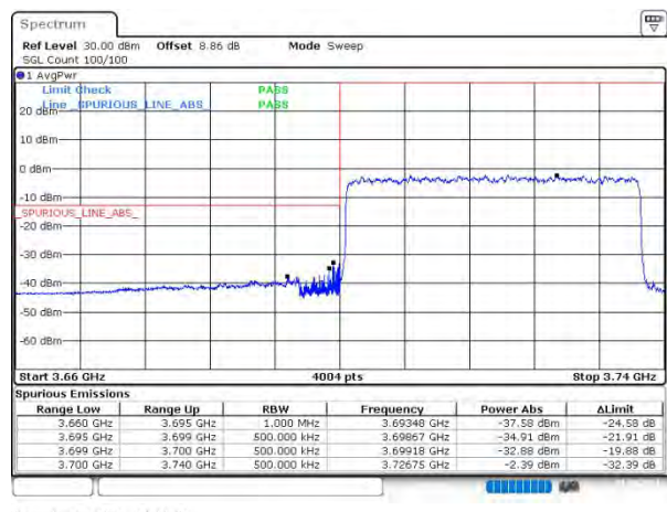
n77(3700-3980) SCS=30kHz DFT_16QAM BW=40MHz LowChannel=648000 RB=100@0
