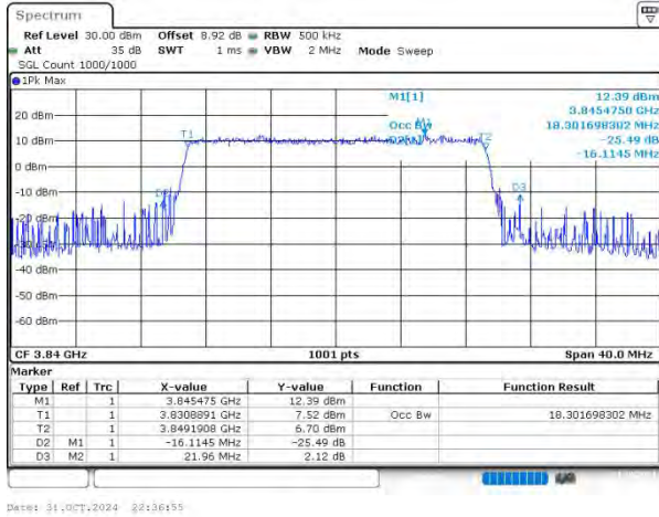
n77(3700-3980) SCS=30kHz CP_256QAM BW=20MHz Channel=656000 RB=51@0
