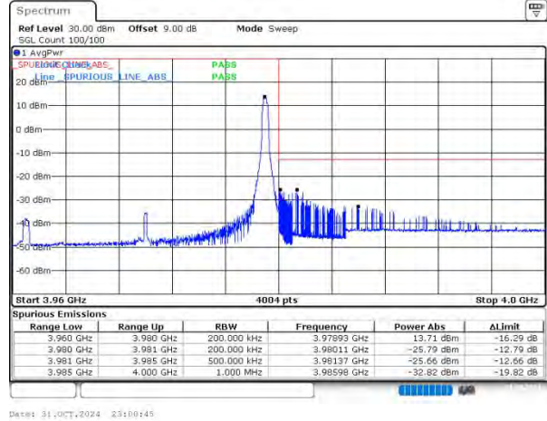
n77(3700-3980) SCS=30kHz DFT_BPSK BW=20MHz HighChannel=664666 RB=1@50
