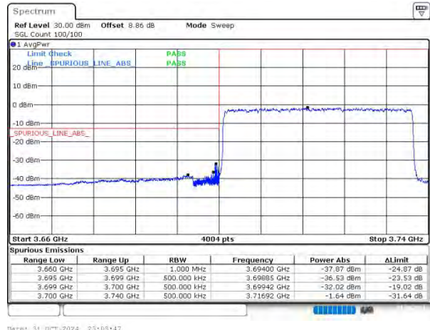
n77(3700-3980) SCS=30kHz DFT_QPSK BW=40MHz LowChannel=648000 RB=100@0
