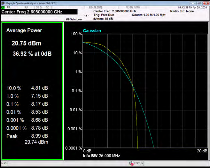
Band41(2555-2655) QPSK BW=15MHz Channel=40740 RB Size=1 Position=#0
