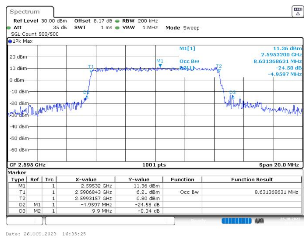
n38 SCS=30kHz CP_QAM64 BW=10MHz Channel=519000 RB=24@0
