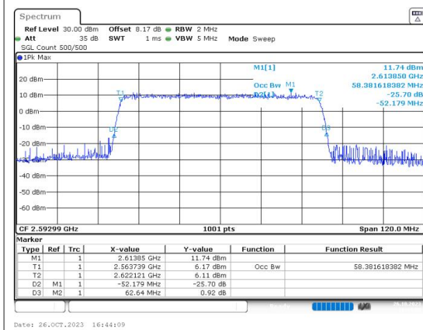
n41 SCS=30kHz CP_QAM256 BW=60MHz Channel=518598 RB=162@0
