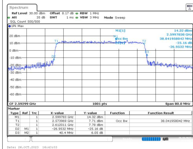
n41 SCS=30kHz CP_QAM16 BW=40MHz Channel=518598 RB=106@0
