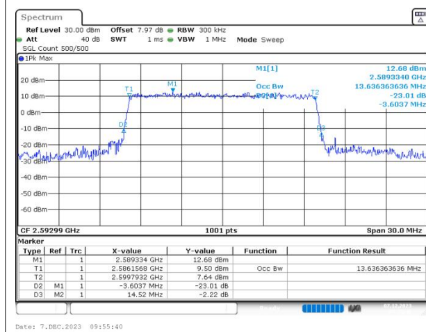
n41 SCS=30kHz CP_64QAM BW=15MHz Channel=518598 RB=38@0
