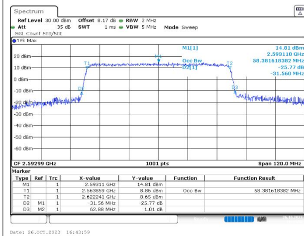
n41 SCS=30kHz CP_QAM16 BW=60MHz Channel=518598 RB=162@0
