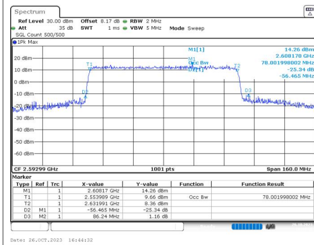
n41 SCS=30kHz CP_QAM64 BW=80MHz Channel=518598 RB=217@0
