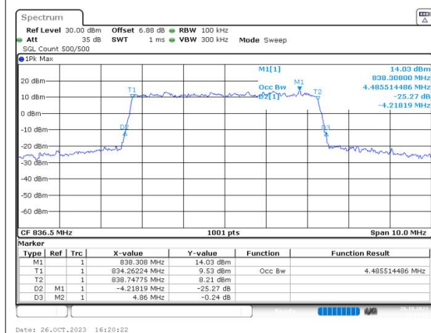
n5 SCS=15kHz CP_QAM16 BW=5MHz Channel=167300 RB=25@0
