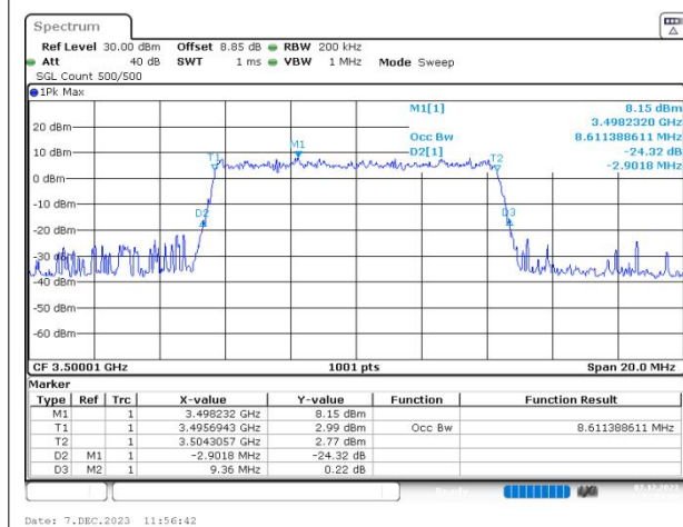
n77(3450-3550) SCS=30kHz CP_256QAM BW=10MHz Channel=633334 RB=24@0
