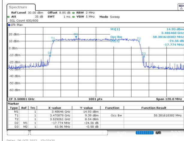
n77(3450-3550) SCS=30kHz CP_QAM64 BW=60MHz Channel=633334 RB=162@0
