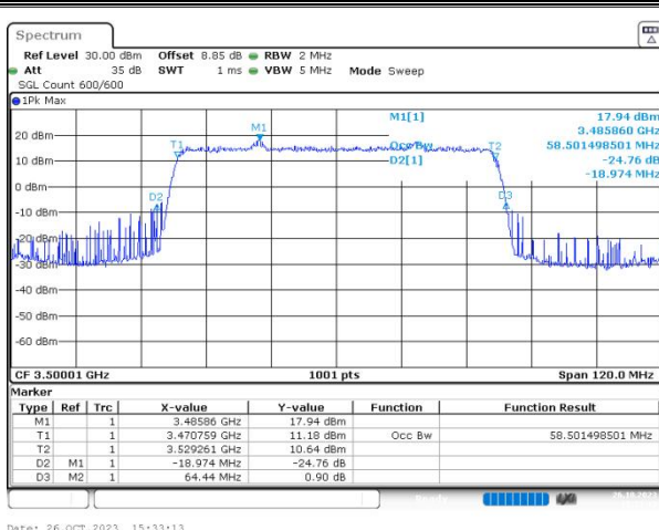
n77(3450-3550) SCS=30kHz DFT_BPSK BW=60MHz Channel=633334 RB=162@0
