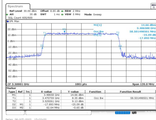
n77(3450-3550) SCS=30kHz CP_QPSK BW=60MHz Channel=633334 RB=162@0
