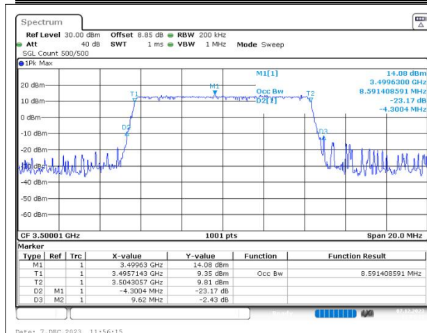
n77(3450-3550) SCS=30kHz DFT_BPSK BW=10MHz Channel=633334 RB=24@0
