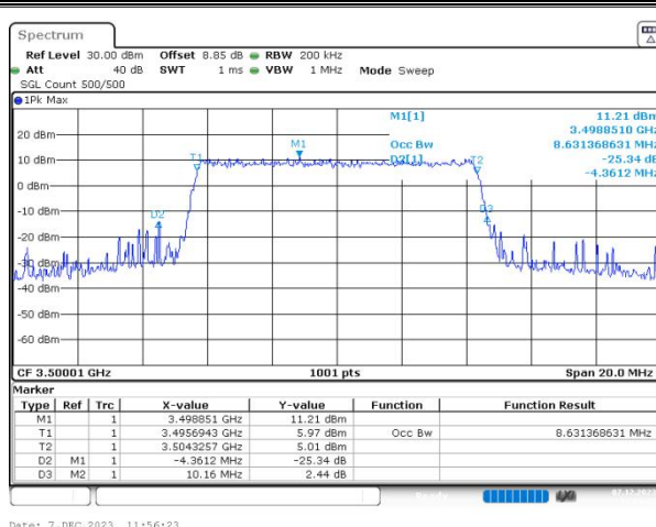
n77(3450-3550) SCS=30kHz CP_QPSK BW=10MHz Channel=633334 RB=24@0
