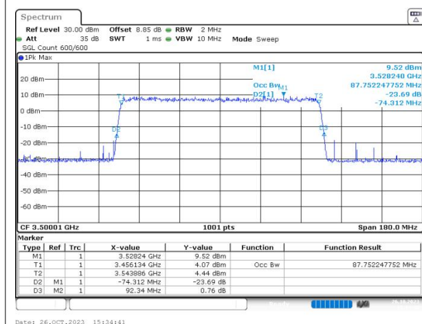
n77(3450-3550) SCS=30kHz CP_QAM256 BW=90MHz Channel=633334 RB=245@0
