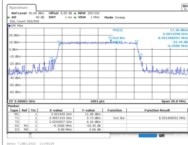
n77(3450-3550) SCS=30kHz CP_16QAM BW=10MHz Channel=633334 RB=24@0
