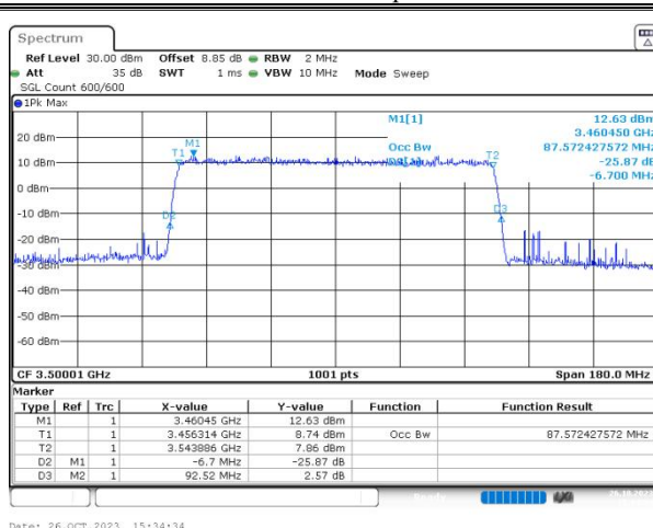
n77(3450-3550) SCS=30kHz CP_QAM64 BW=90MHz Channel=633334 RB=245@0
