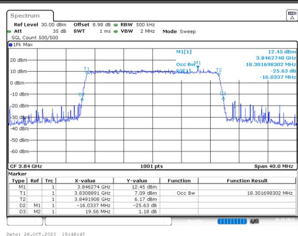
n77(3700-3980) SCS=30kHz CP_QAM64 BW=20MHz Channel=656000 RB=51@0
