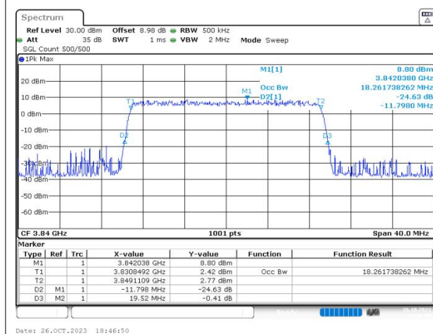
n77(3700-3980) SCS=30kHz CP_QAM256 BW=20MHz Channel=656000 RB=51@0
