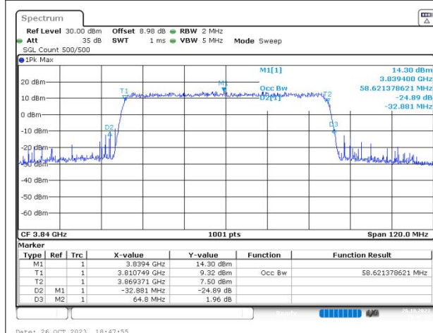
n77(3700-3980) SCS=30kHz CP_QAM64 BW=60MHz Channel=656000 RB=162@0
