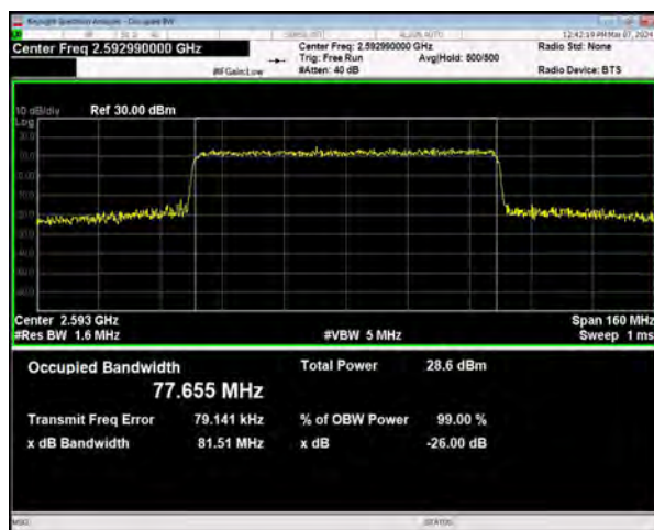
n41 SCS=30kHz CP_16QAM BW=80MHz Channel=518598 RB=217@0
