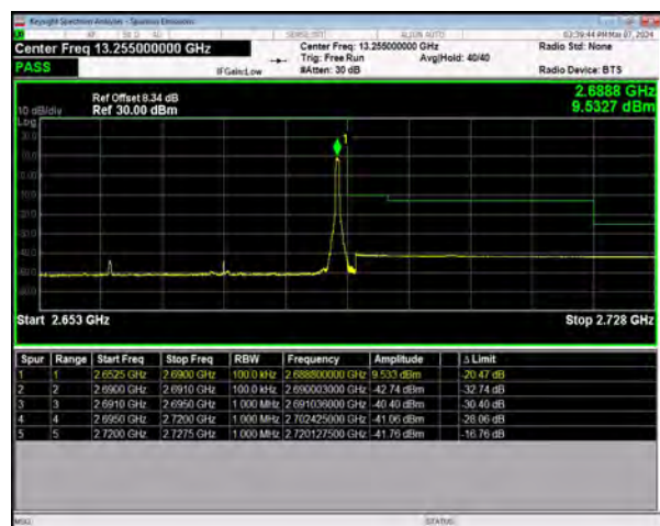
n41 SCS=30kHz DFT_BPSK BW=30MHz HighChannel=534996
