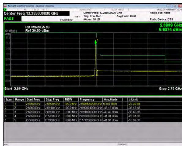
n41 SCS=30kHz DFT_16QAM BW=80MHz HighChannel=529998 RB=1@216
