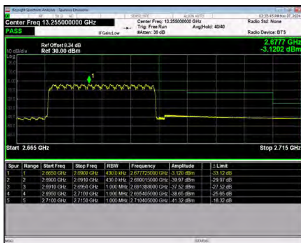
n41 SCS=30kHz CP_QPSK BW=20MHz HighChannel=535998
