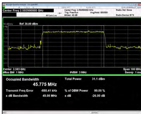
n41 SCS=30kHz DFT_BPSK BW=50MHz Channel=518598 RB=128@0
