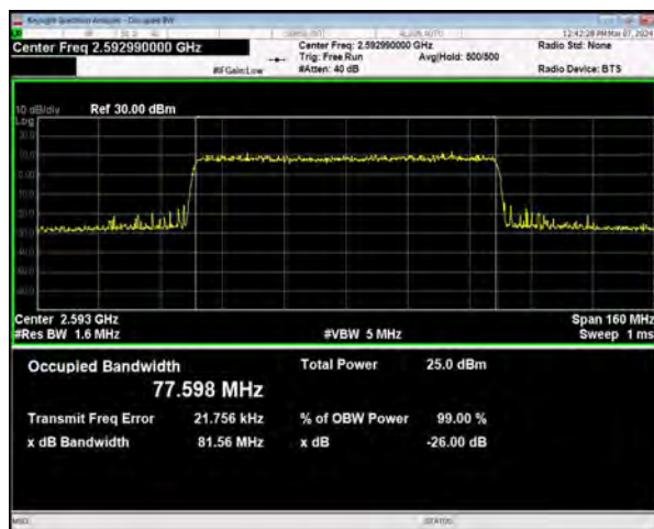
n41 SCS=30kHz CP_256QAM BW=80MHz Channel=518598 RB=217@0
