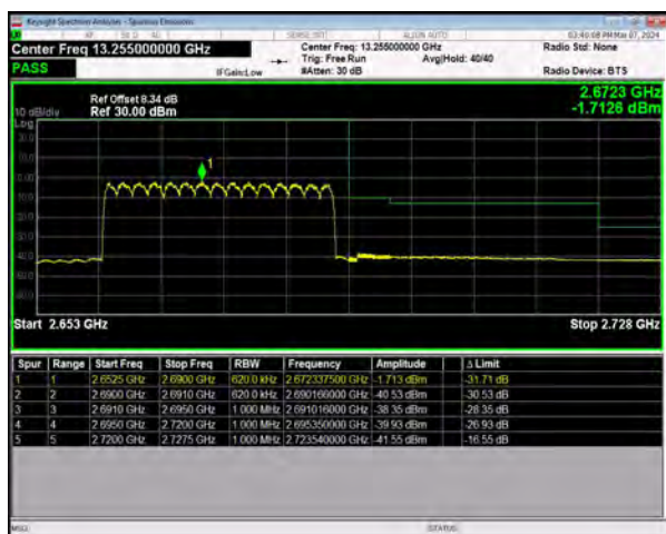
n41 SCS=30kHz DFT_BPSK BW=30MHz HighChannel=534996 RB=75@0
