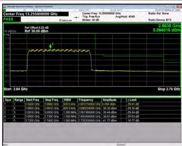
n41 SCS=30kHz DFT_BPSK BW=40MHz HighChannel=534000
