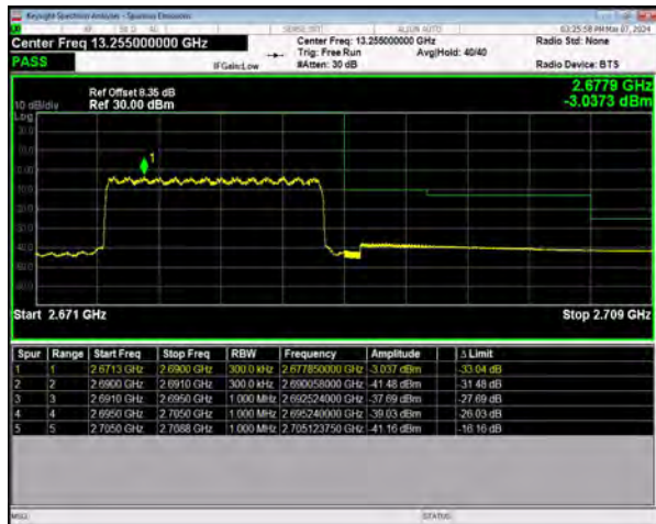
n41 SCS=30kHz DFT_16QAM BW=15MHz HighChannel=536496 RB=36@0
