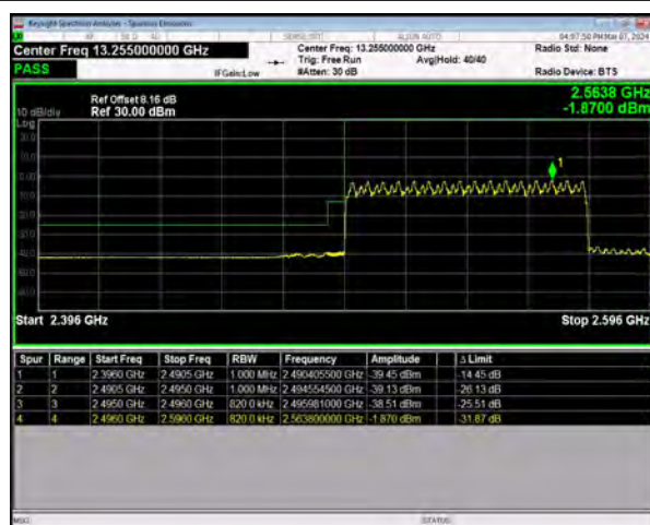
n41 SCS=30kHz DFT_BPSK BW=80MHz LowChannel=507204
