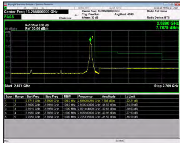
n41 SCS=30kHz DFT_64QAM BW=15MHz HighChannel=536496 RB=1@37
