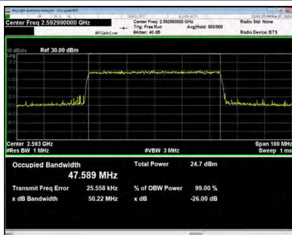
n41 SCS=30kHz CP_256QAM BW=50MHz Channel=518598 RB=133@0
