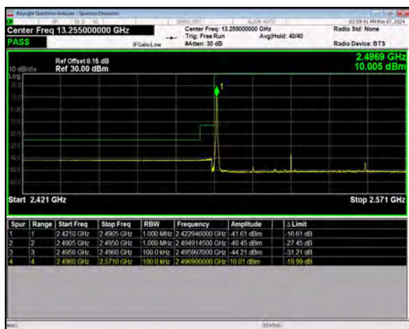
n41 SCS=30kHz DFT_BPSK BW=60MHz LowChannel=505200 RB=1@0
