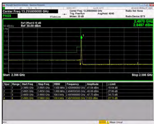
n41 SCS=30kHz DFT_256QAM BW=80MHz LowChannel=507204 RB=1@0
