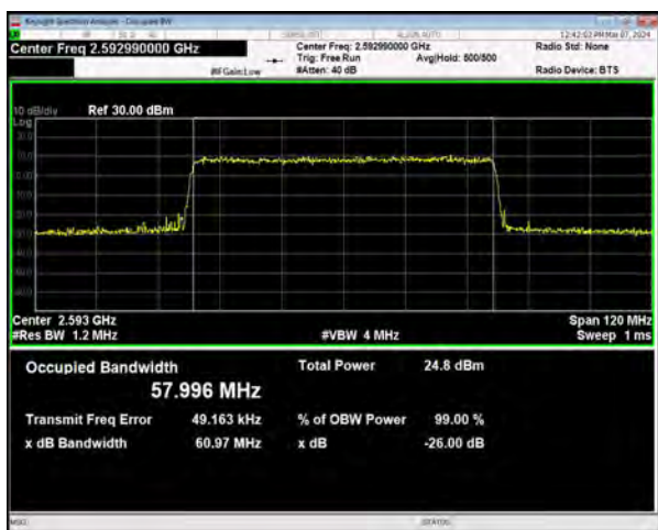
n41 SCS=30kHz CP_256QAM BW=60MHz Channel=518598 RB=162@0
