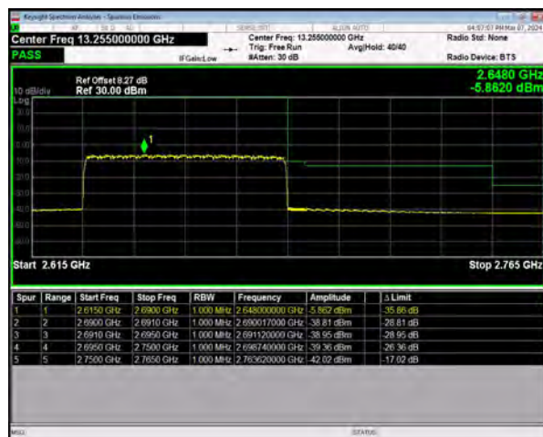
n41 SCS=30kHz CP_QPSK BW=60MHz HighChannel=531996
