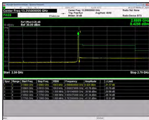
n41 SCS=30kHz DFT_BPSK BW=80MHz HighChannel=529998 RB=1@216
