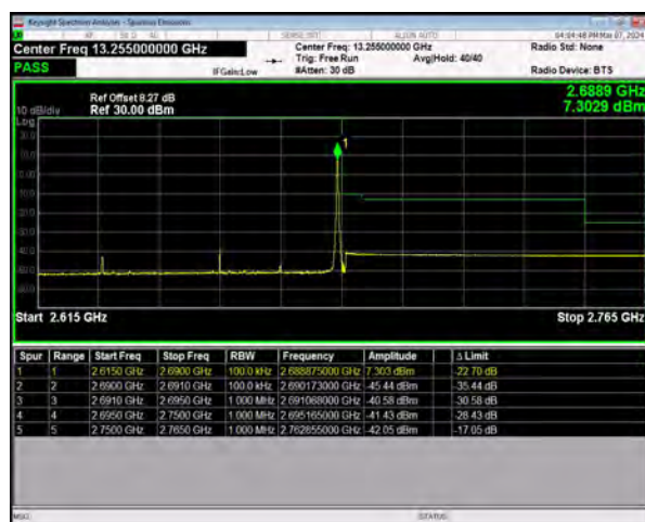
n41 SCS=30kHz DFT_16QAM BW=60MHz HighChannel=531996 RB=1@161
