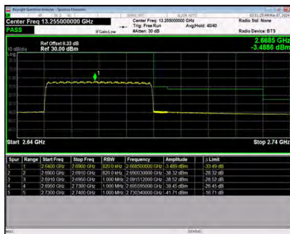
n41 SCS=30kHz CP_QPSK BW=40MHz HighChannel=534000 RB=106@0
