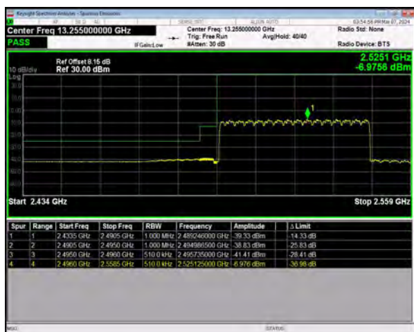
n41 SCS=30kHz CP_QPSK BW=50MHz LowChannel=504204 RB=133@0
