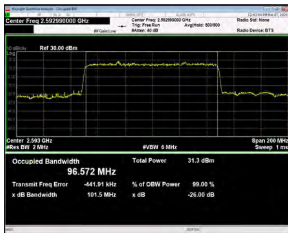
n41 SCS=30kHz DFT_BPSK BW=100MHz Channel=518598 RB=270@0
