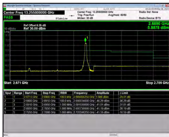
n41 SCS=30kHz DFT_256QAM BW=15MHz HighChannel=536496 RB=1@37
