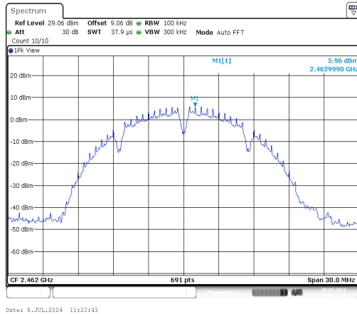
11B-Ant1-2462-0~Reference-PASS
