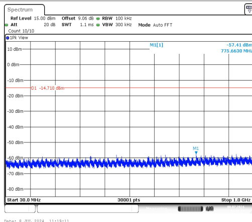
11B-Ant1-2437-30~1000-PASS
