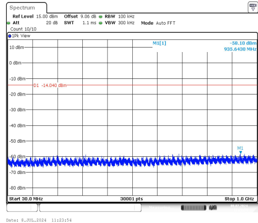
11B-Ant1-2462-30~1000-PASS
