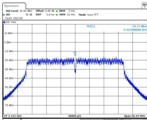
11N20SISO-Ant1-2412-PASS
