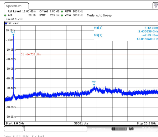
11B-Ant1-2437-1000~26500-PASS
