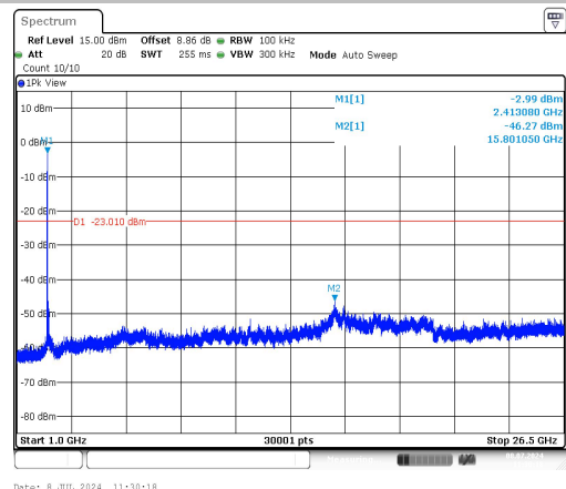
11G-Ant1-2412-1000~26500-PASS
