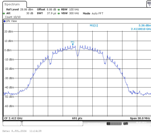
11B-Ant1-2412-0~Reference-PASS
