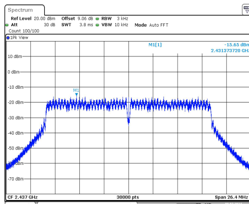
11N20SISO-Ant1-2437-PASS
