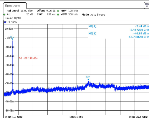
11G-Ant1-2462-0~Reference-PASS
