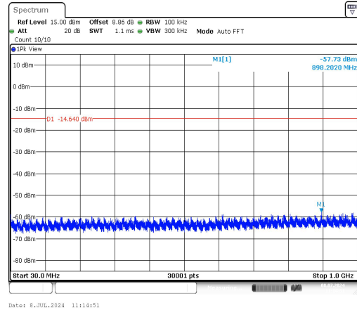
11B-Ant1-2412-30~1000-PASS
