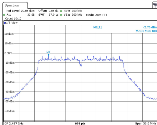
11G-Ant1-2437-0~Reference-PASS
