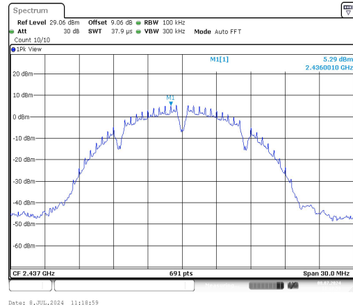
11B-Ant1-2437-0~Reference-PASS
