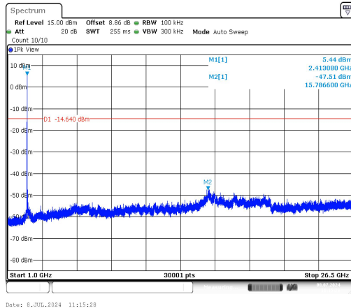
11B-Ant1-2412-1000~26500-PASS
