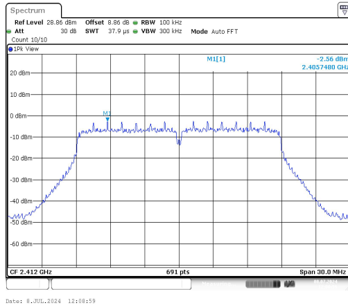
11N20SISO-Ant1-2412-0~Reference-PASS
