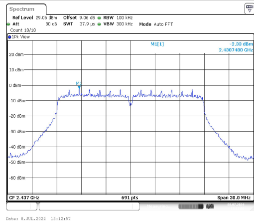
11N20SISO-Ant1-2437-0~Reference-PASS
