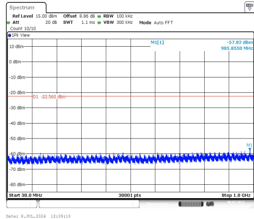
11N20SISO-Ant1-2412-30~1000-PASS
