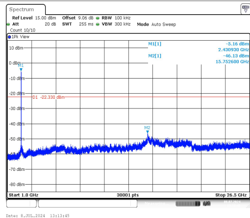
11N20SISO-Ant1-2437-1000~26500-PASS
