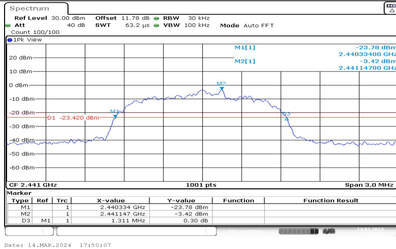
3DH5-Ant1-2441
