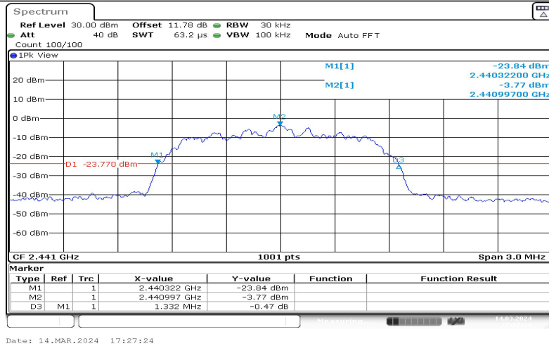
2DH5-Ant1-2441
