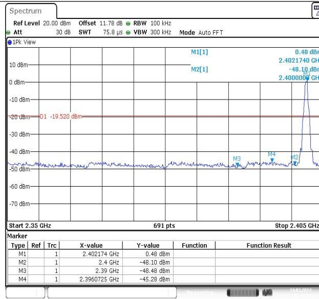
DH5-Ant1-2402-PASS
