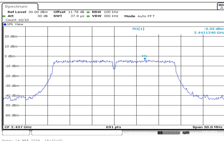
11G-Ant1-2437-0~Reference--3.35
