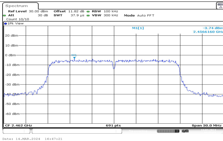
11N20SISO-Ant1-2462-0~Reference--3.74
