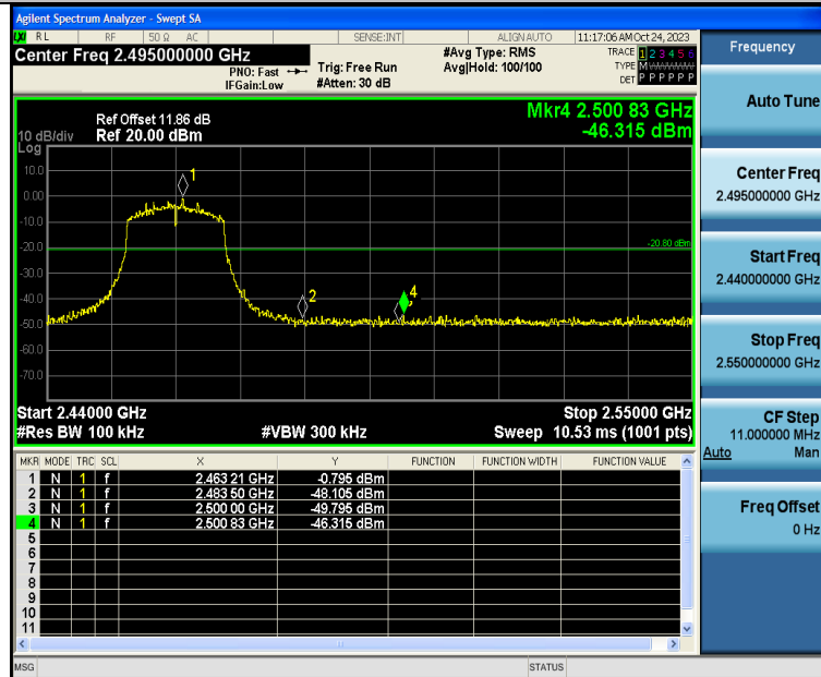
11G-Ant1-2462-PASS
