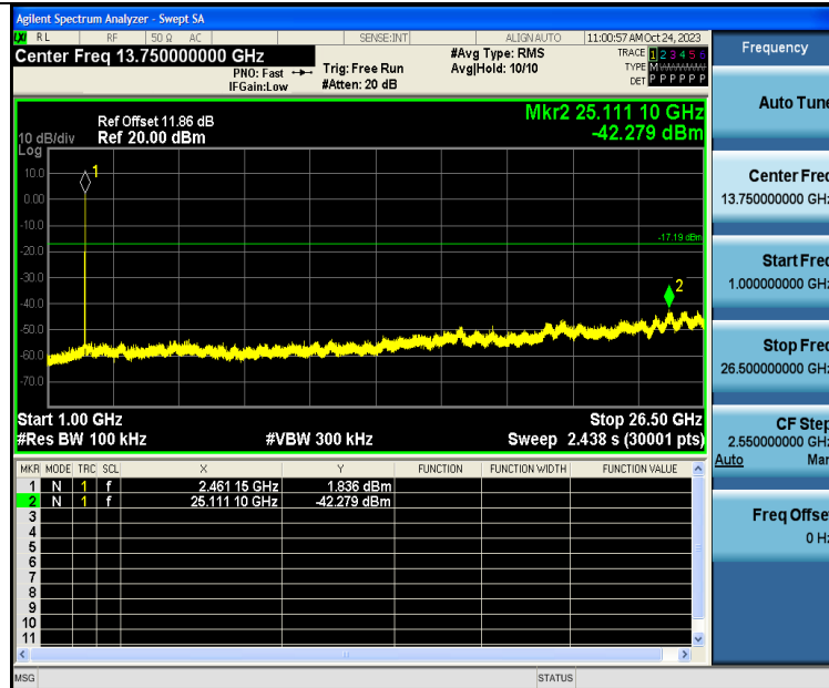
11B-Ant1-2462-1000~26500-PASS
