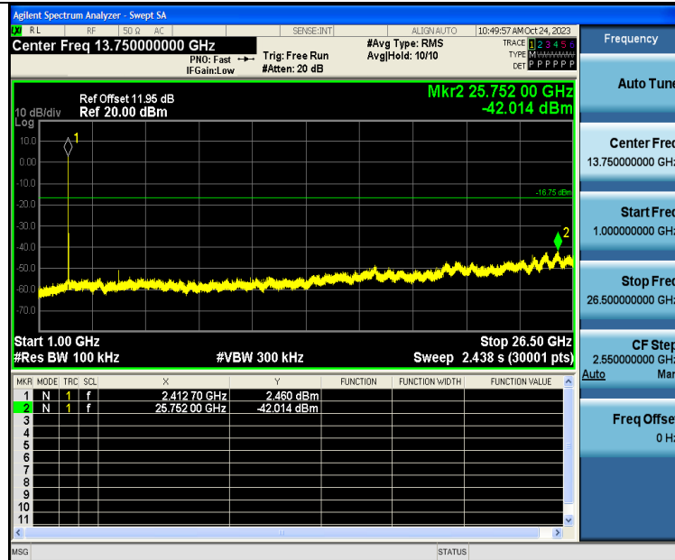
11B-Ant1-2412-1000~26500-PASS
