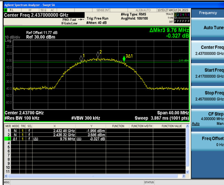
11B-Ant1-2437-PASS
