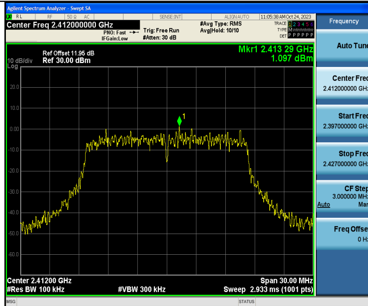
11G-Ant1-2412-0~Reference-PASS
