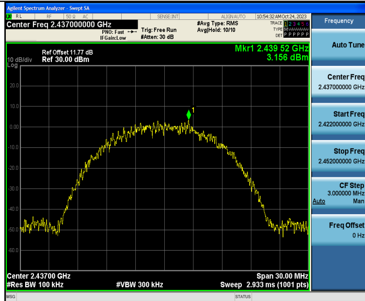
11B-Ant1-2437-0~Reference-PASS
