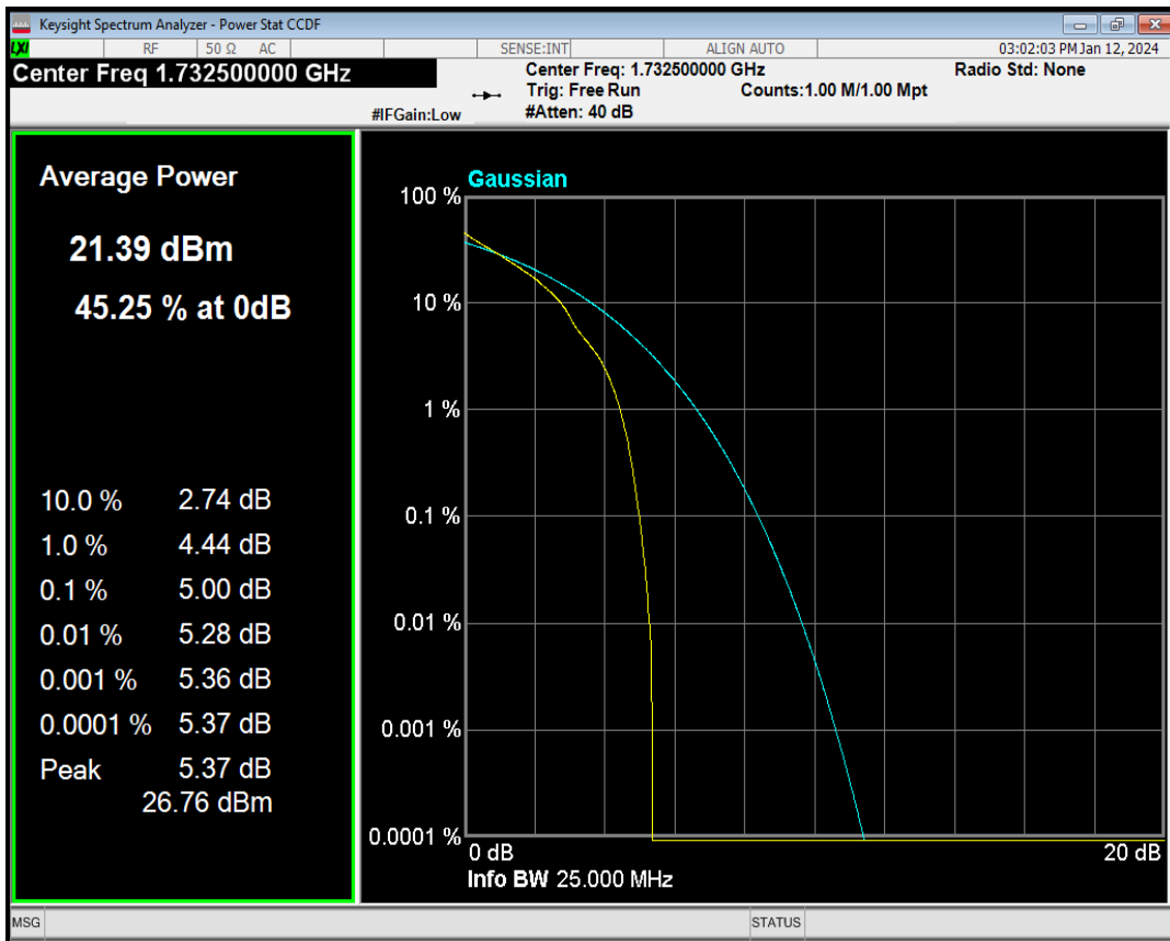
Band4 QPSK BW=15MHz Channel=20175 RB Size=1 Position=#Max
