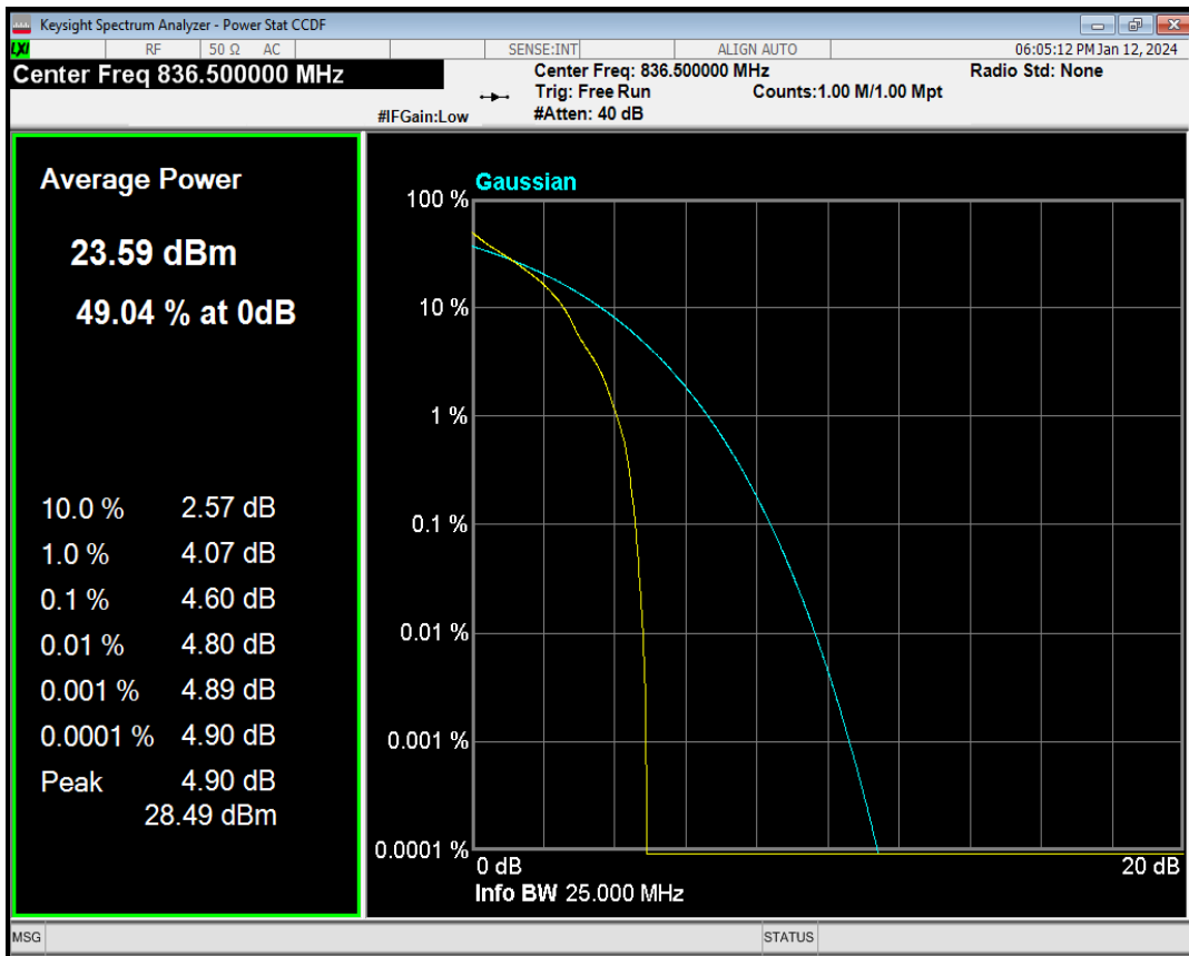
Band5 QPSK BW=1.4MHz Channel=20525 RB Size=1 Position=#Max
