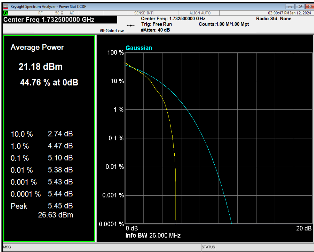
Band4 QPSK BW=10MHz Channel=20175 RB Size=1 Position=#Max
