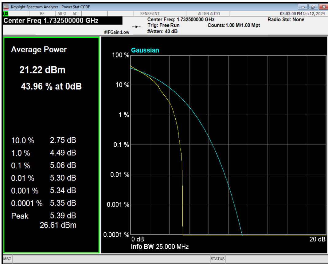
Band4 QPSK BW=20MHz Channel=20175 RB Size=1 Position=#Max
