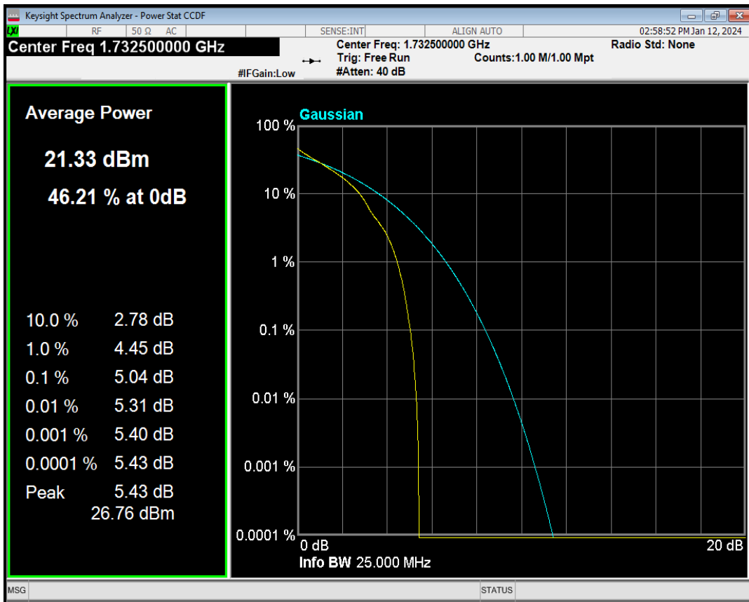
Band4 QPSK BW=3MHz Channel=20175 RB Size=1 Position=#Max
