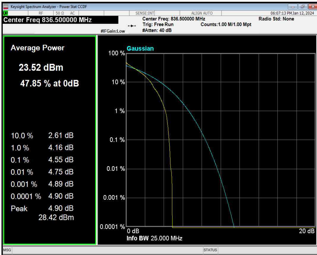
Band5 QPSK BW=5MHz Channel=20525 RB Size=1 Position=#Max
