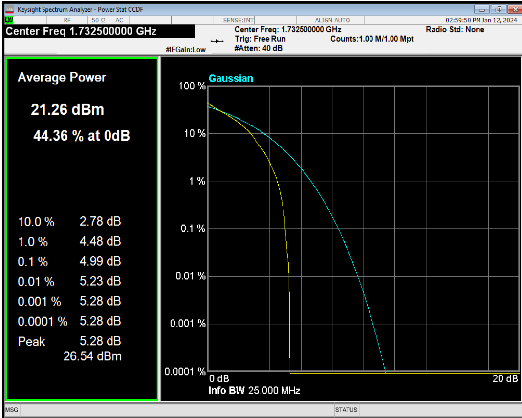
Band4 QPSK BW=5MHz Channel=20175 RB Size=1 Position=#Max
