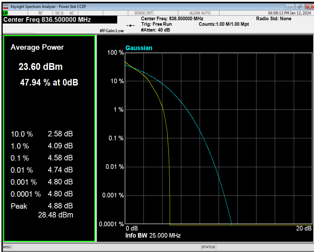
Band5 QPSK BW=10MHz Channel=20525 RB Size=1 Position=#Max
